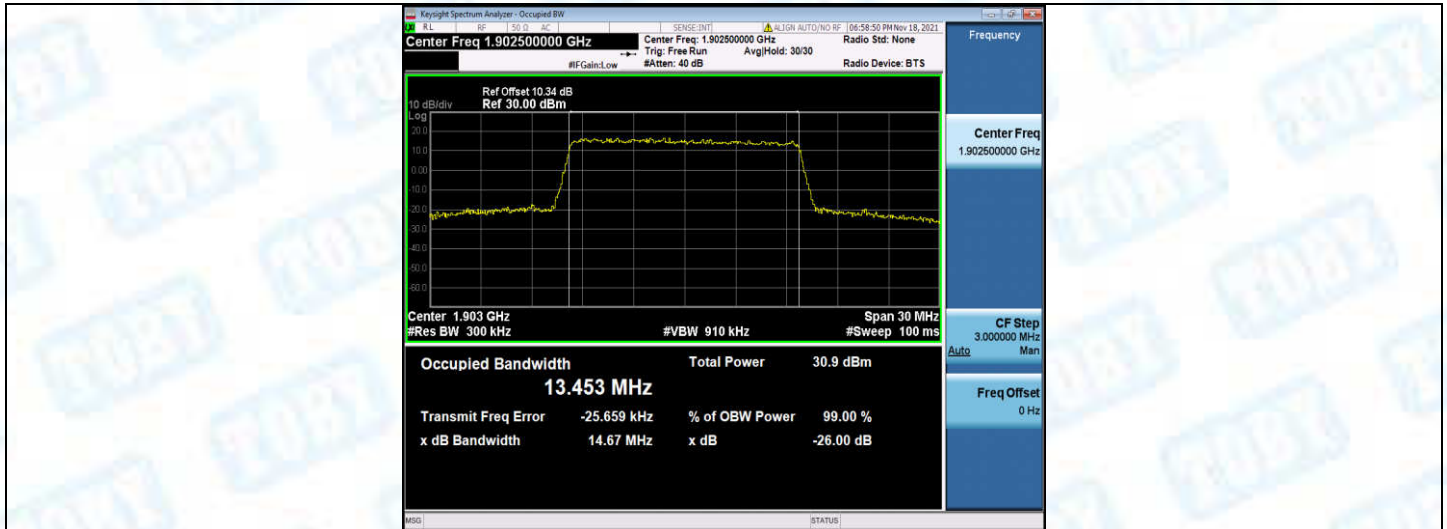
Band2-15MHz-16QAM-18675-75RB#0
