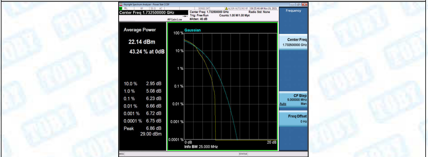
Band4-15MHz-16QAM-20175-75RB#0
