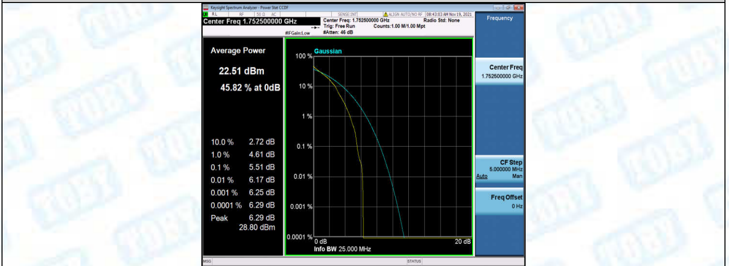
Band4-5MHz-QPSK-20375-25RB#0
