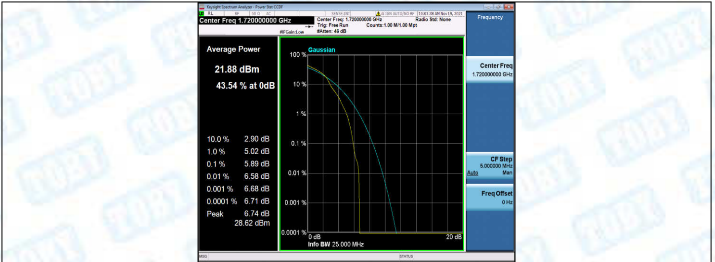
Band4-20MHz-16QAM-20050-100RB#0
