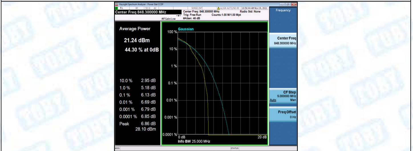
Band5-1.4MHz-16QAM-20643-6RB#0
