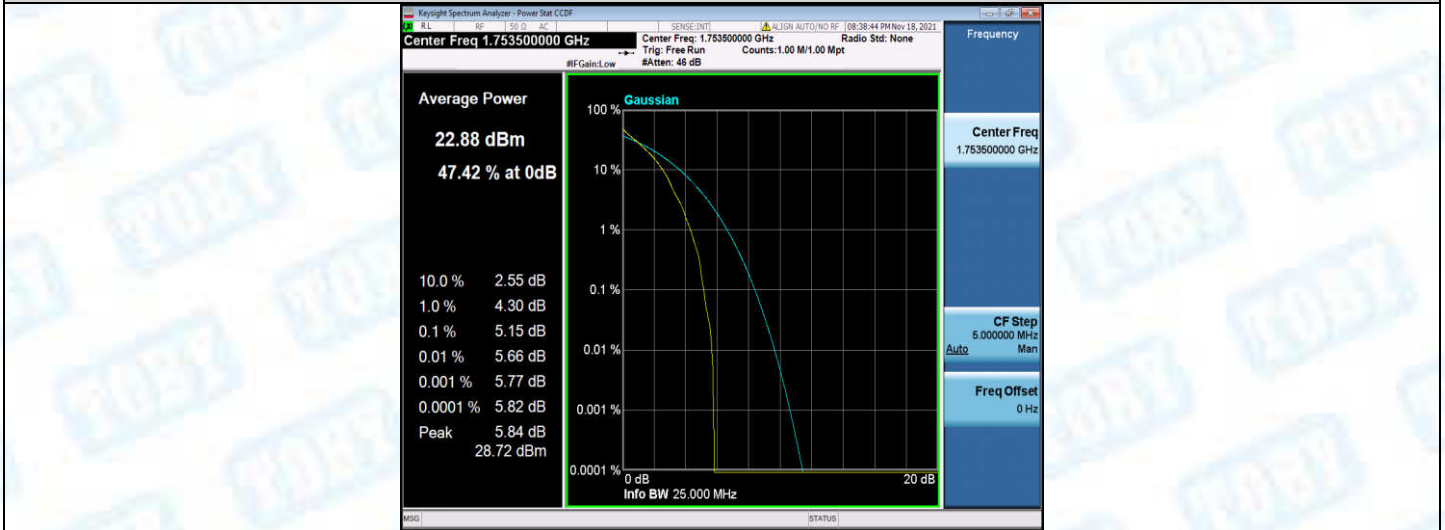
Band4-3MHz-QPSK-20385-15RB#0
