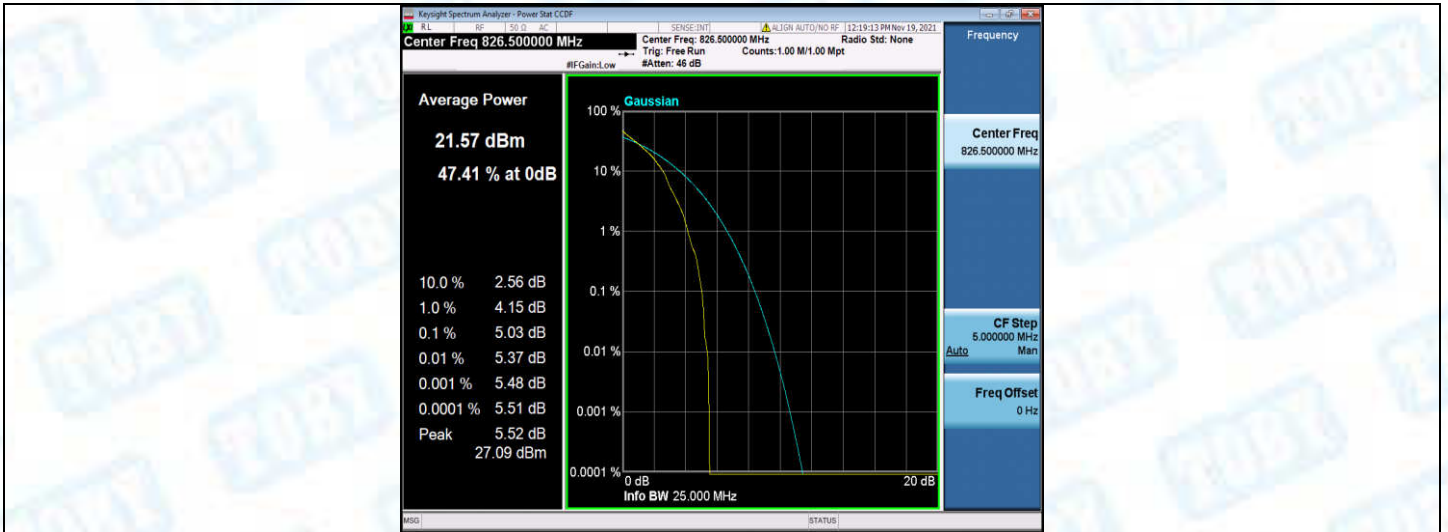
Band5-5MHz-QPSK-20425-25RB#0
