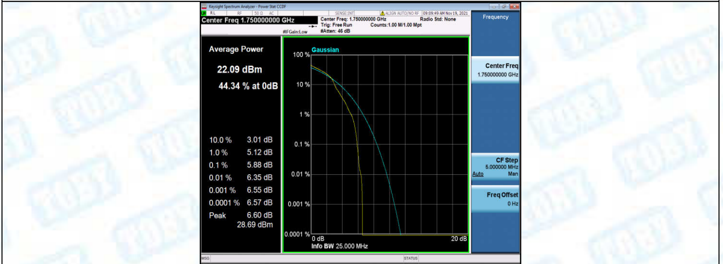
Band4-10MHz-16QAM-20350-50RB#0
