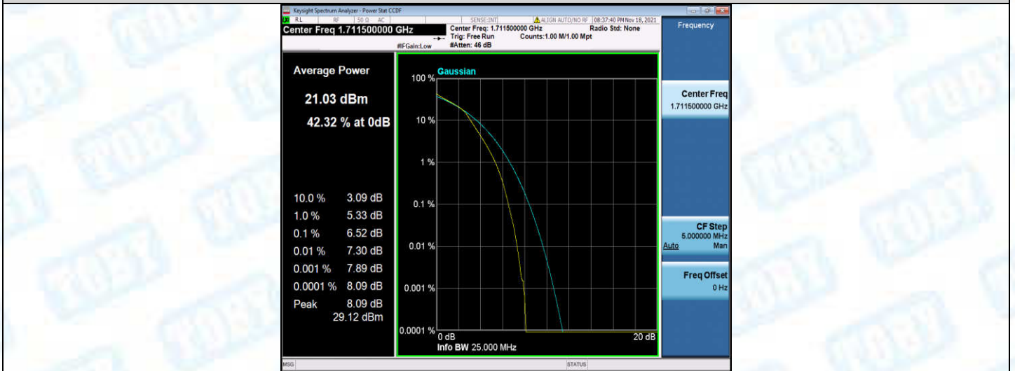
Band4-3MHz-16QAM-20175-1RB#0
