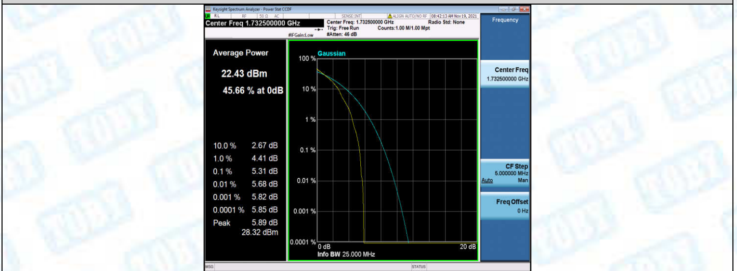
Band4-5MHz-QPSK-20175-25RB#0
