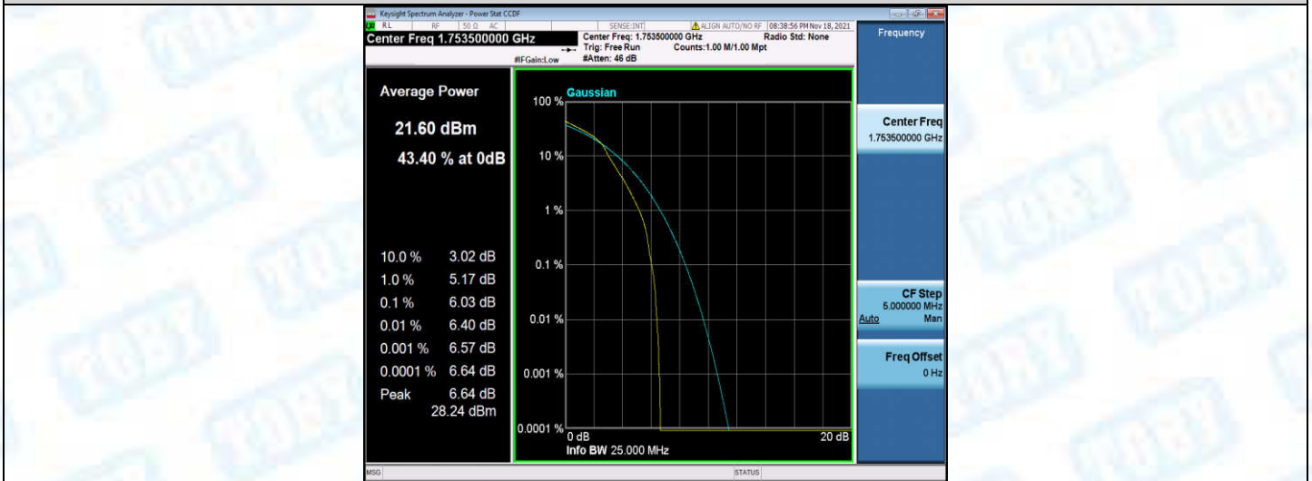
Band4-3MHz-16QAM-20385-15RB#0
