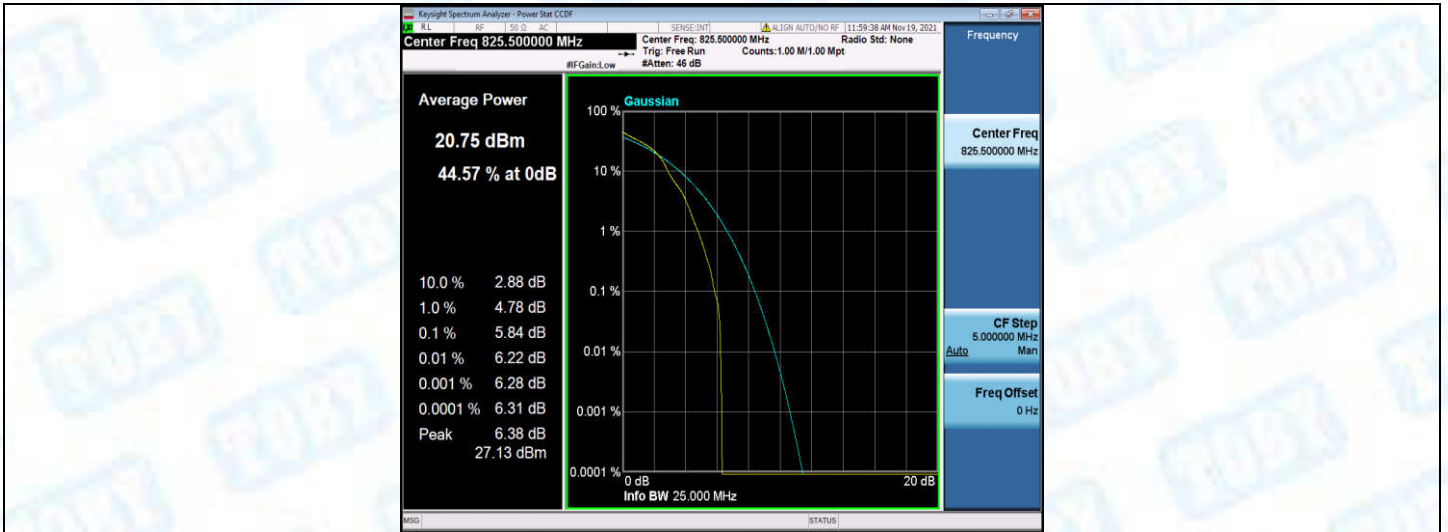
Band5-3MHz-16QAM-20415-15RB#0
