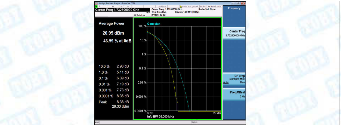
Band4-20MHz-16QAM-20300-1RB#0
