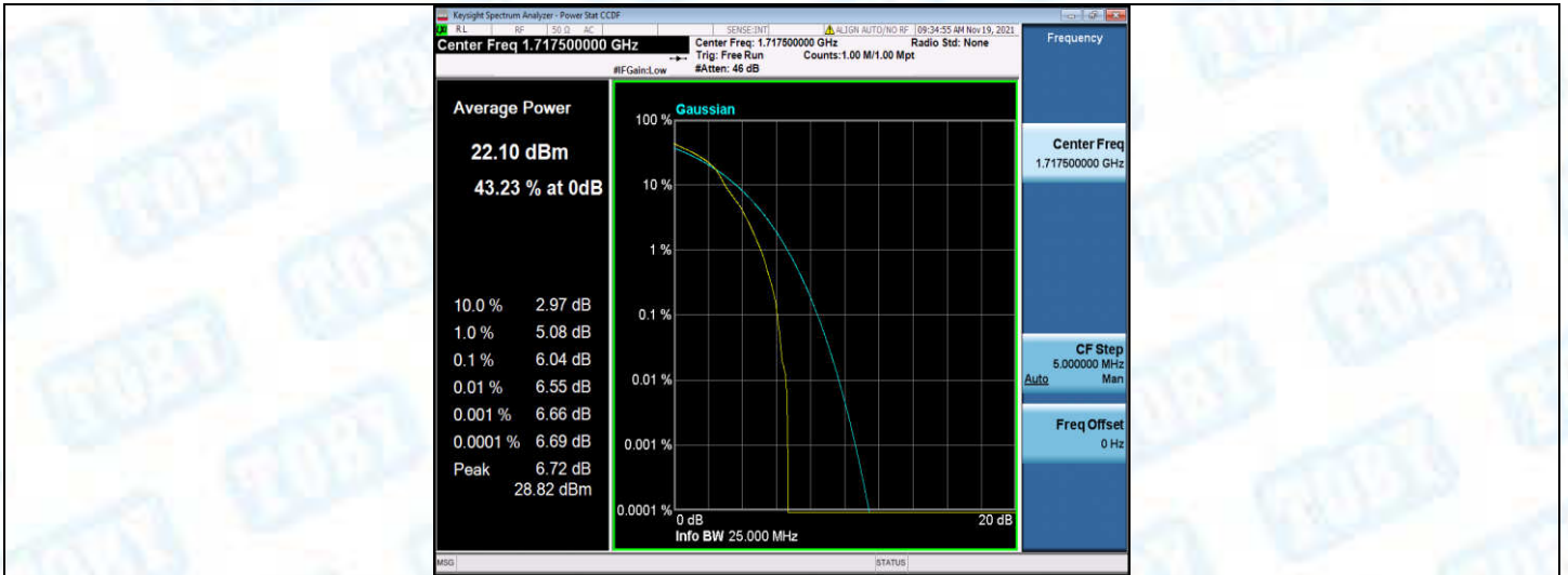
Band4-15MHz-16QAM-20025-75RB#0
