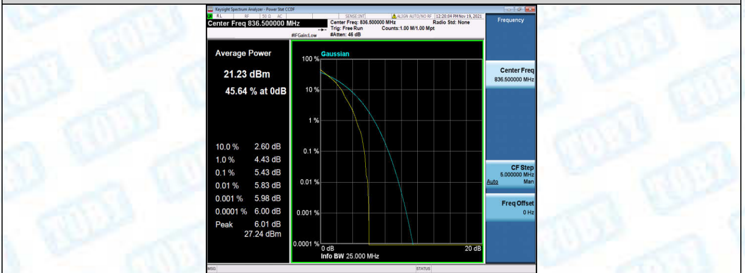
Band5-5MHz-QPSK-20525-25RB#0
