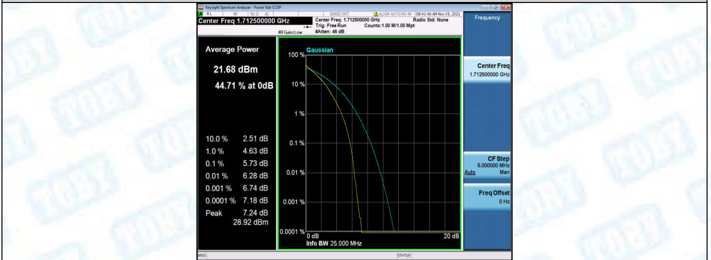
Band4-5MHz-QPSK-20175-1RB#0
