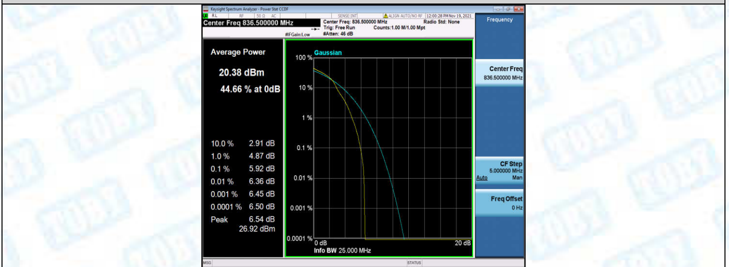
Band5-3MHz-16QAM-20525-15RB#0
