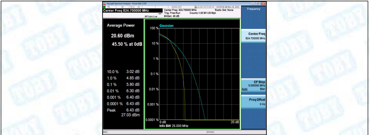
Band5-1.4MHz-16QAM-20407-6RB#0
