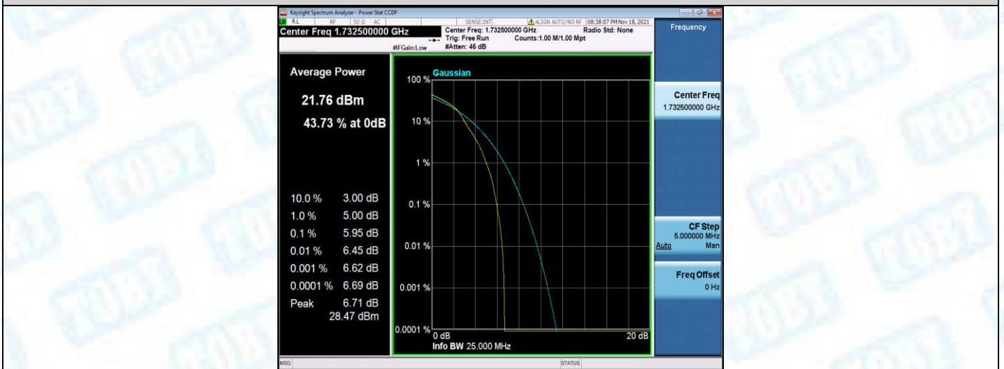
Band4-3MHz-16QAM-20175-15RB#0
