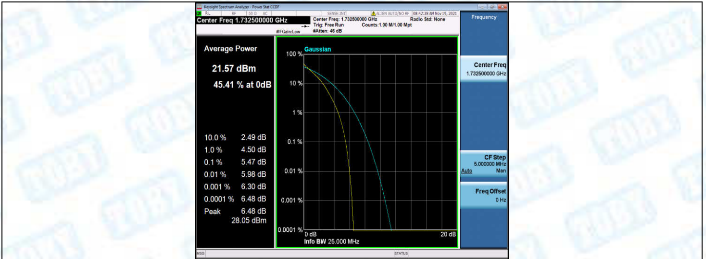
Band4-5MHz-QPSK-20375-1RB#0
