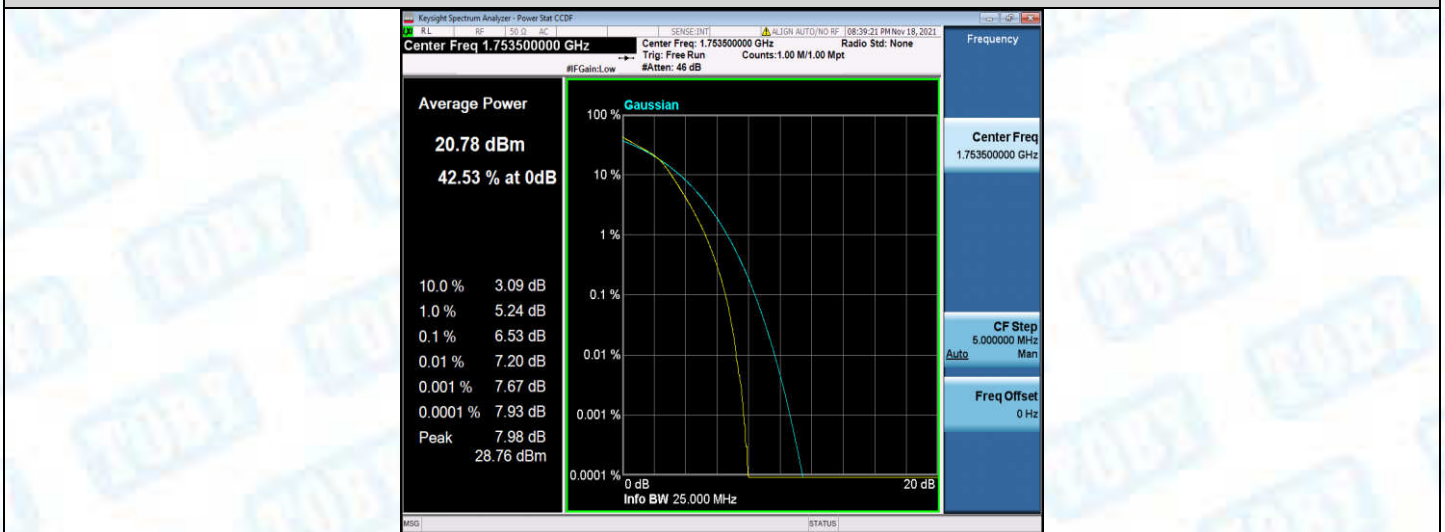
Band4-5MHz-QPSK-19975-1RB#0
