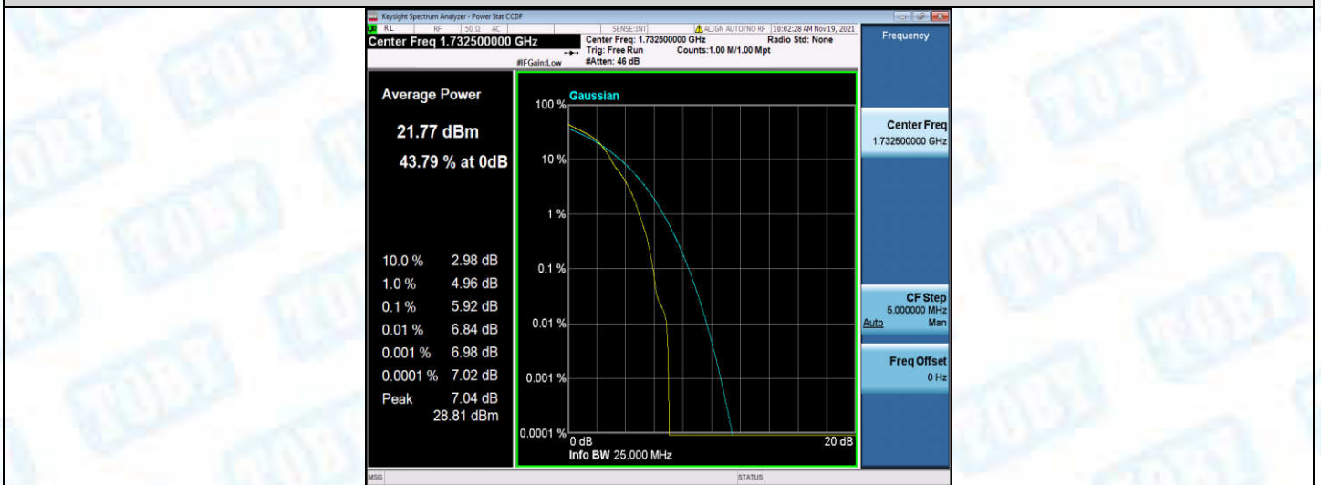
Band4-20MHz-16QAM-20175-100RB#0
