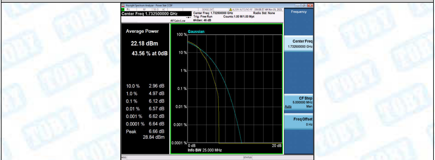
Band4-10MHz-16QAM-20175-50RB#0
