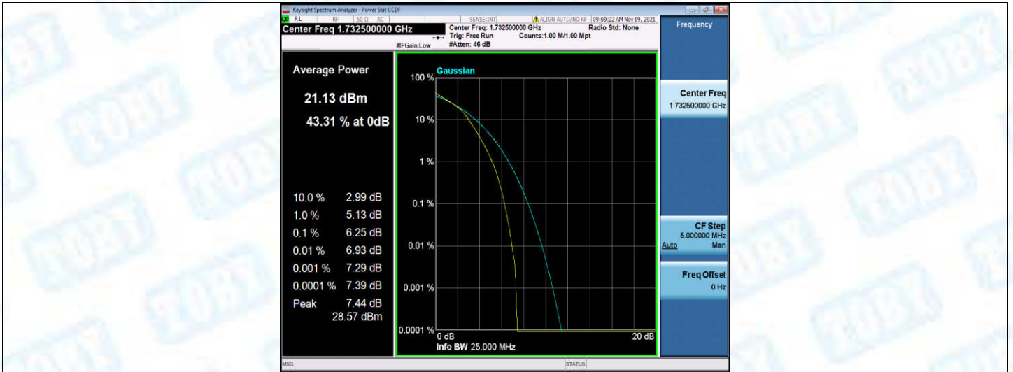
Band4-10MHz-16QAM-20350-1RB#0
