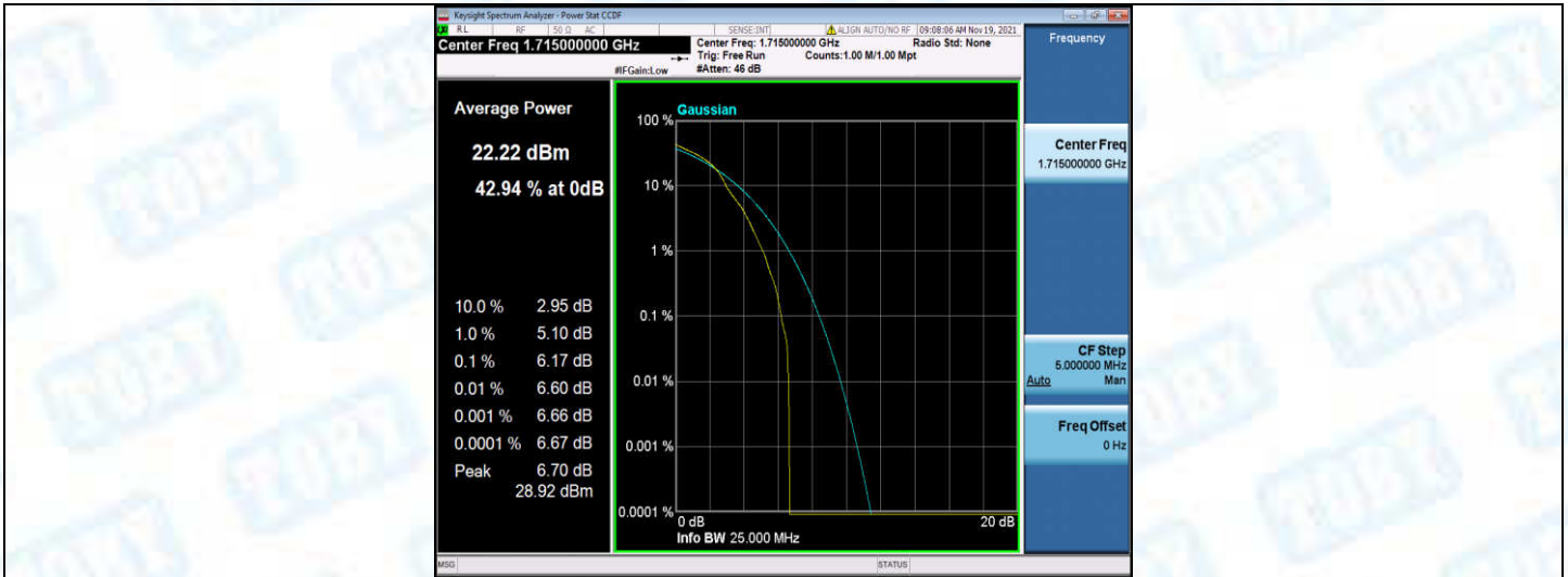
Band4-10MHz-16QAM-20000-50RB#0
