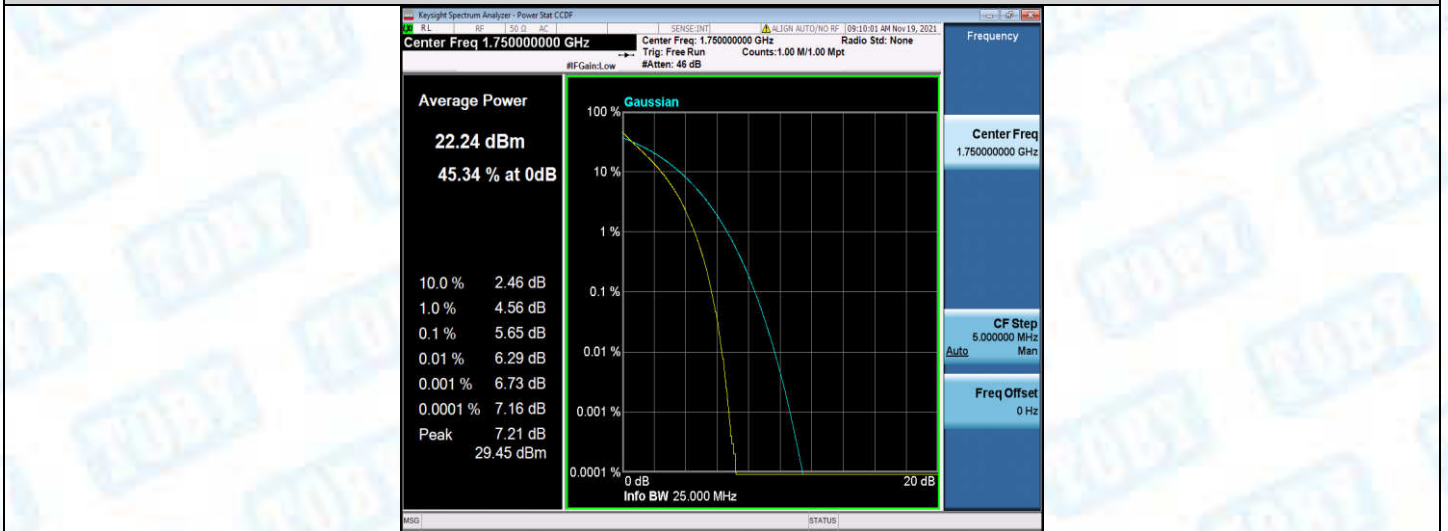
Band4-10MHz-16QAM-20000-1RB#0
