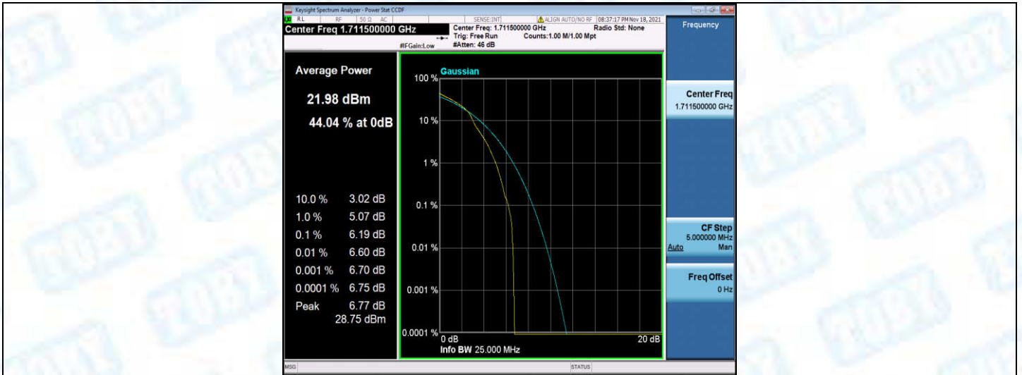
Band4-3MHz-16QAM-19965-15RB#0
