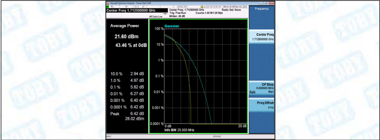
Band4-5MHz-16QAM-19975-25RB#0
