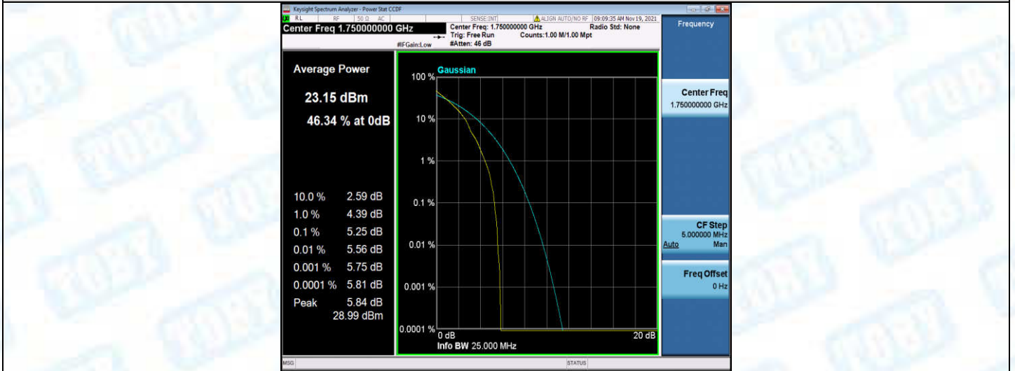
Band4-10MHz-QPSK-20350-50RB#0
