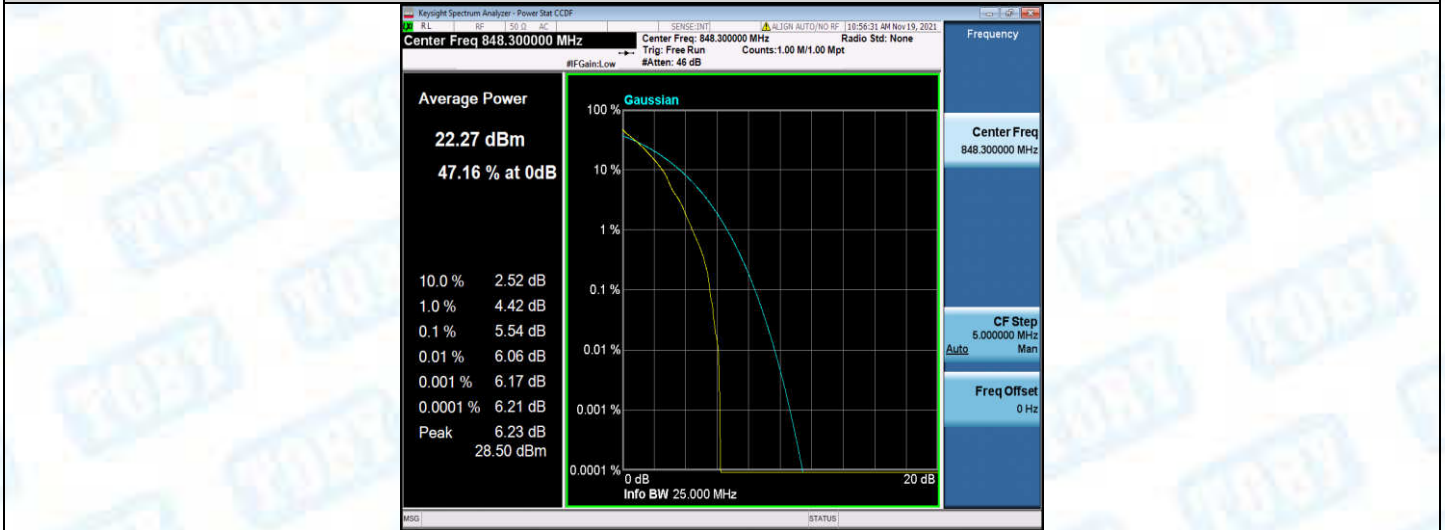
Band5-1.4MHz-QPSK-20643-6RB#0
