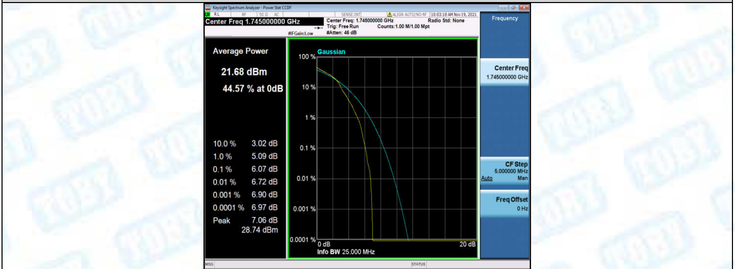
Band4-20MHz-16QAM-20300-100RB#0
