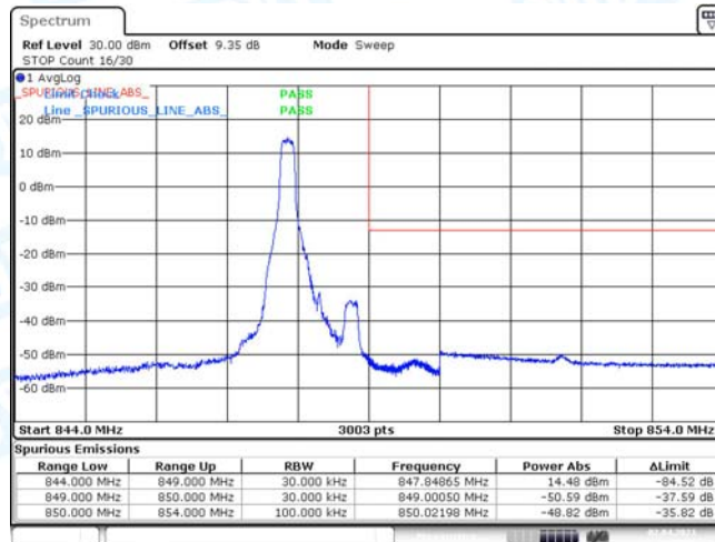
Band5-1.4MHz-QPSK-20643-1RB#0
