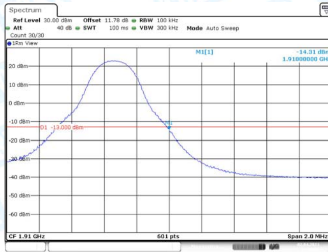
Band2-5MHz-16QAM-19175-1RB#24
