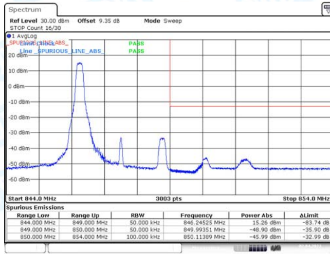
Band5-3MHz-16QAM-20635-1RB#0
