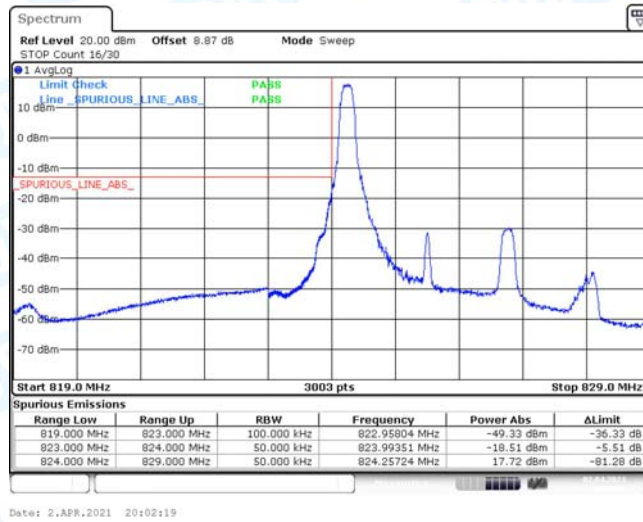
Band5-3MHz-QPSK-20415-15RB#0
