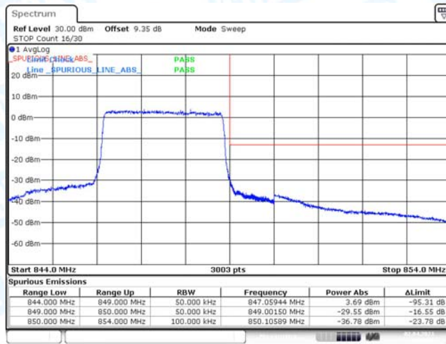
Band5-3MHz-16QAM-20635-15RB#0
