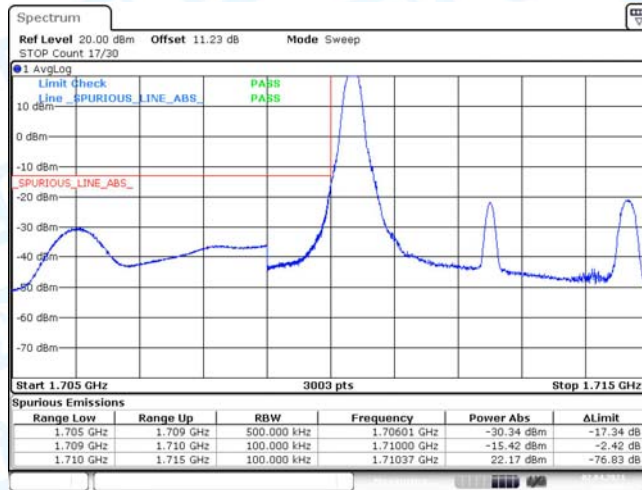
Band4-5MHz-QPSK-19975-25RB#0
