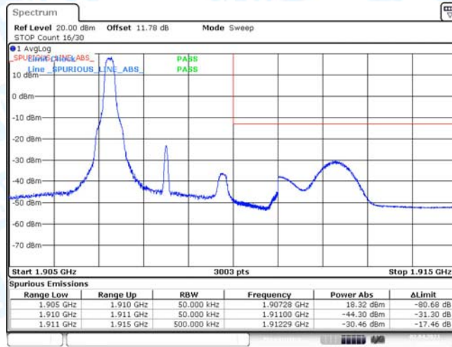
Band2-3MHz-16QAM-19185-1RB#0
