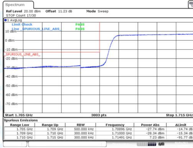
Band4-15MHz-16QAM-20325-1RB#0
