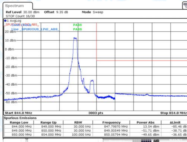
Band5-1.4MHz-16QAM-20643-1RB#0
