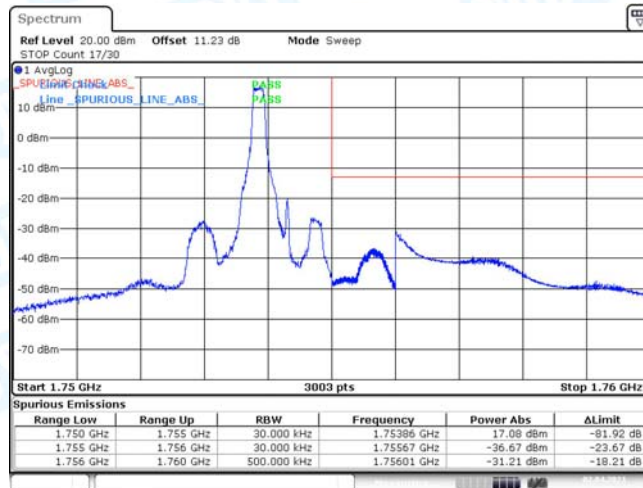
Band4-1.4MHz-QPSK-20393-1RB#0
