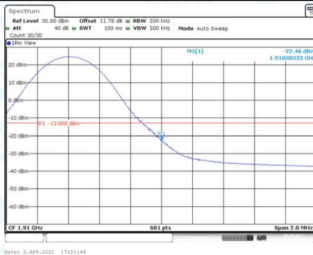
Band2-10MHz-16QAM-19150-50RB#0
