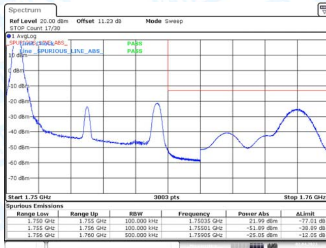
Band4-5MHz-QPSK-20375-1RB#0
