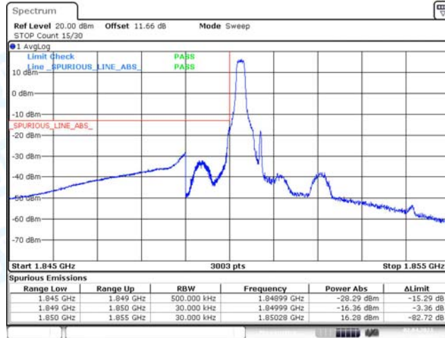
Band2-1.4MHz-16QAM-18607-1RB#0
