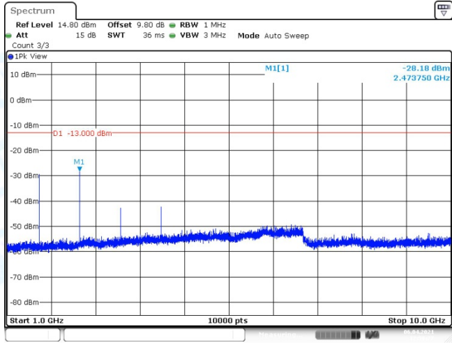
Band5-10MHz-QPSK-20450-1RB#0-Range2:1000~10000MHz
