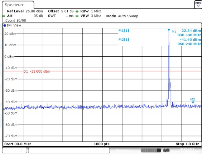
Band5-10MHz-QPSK-20600-1RB#0-Range1:30~1000MHz
