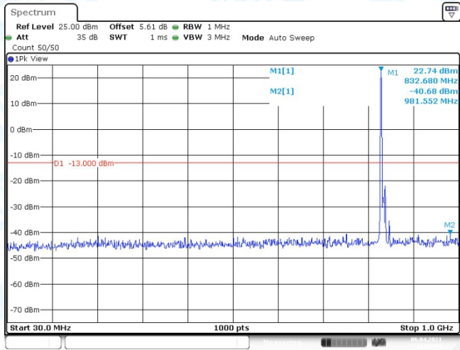
Band5-10MHz-QPSK-20525-1RB#0-Range1:30~1000MHz
