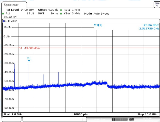
Band5-10MHz-QPSK-20600-1RB#0-Range2:1000~10000MHz
