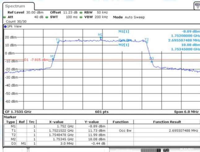
Band4-3MHz-16QAM-20385-15RB#0
