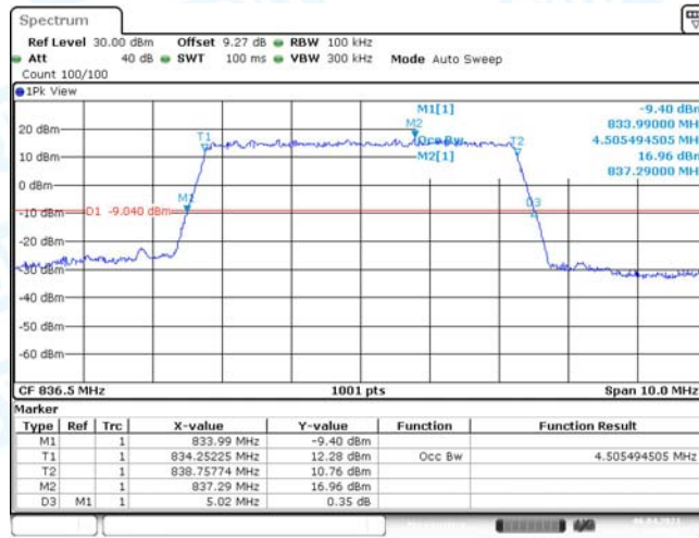
Band5-5MHz-QPSK-20525-25RB#0
