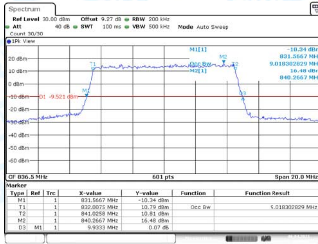
Band5-10MHz-16QAM-20525-50RB#0
