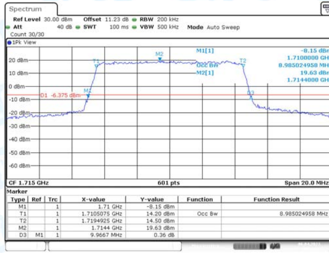
Band4-10MHz-QPSK-20175-50RB#0
