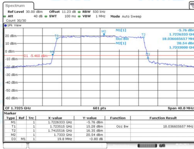
Band4-20MHz-16QAM-20175-100RB#0
