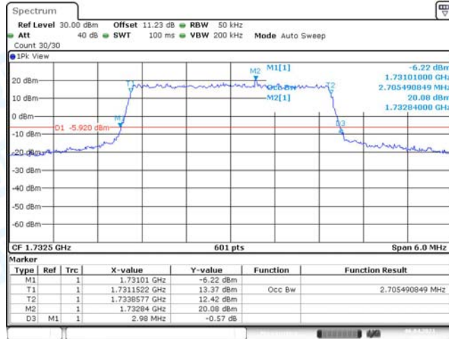
Band4-3MHz-QPSK-20175-15RB#0
