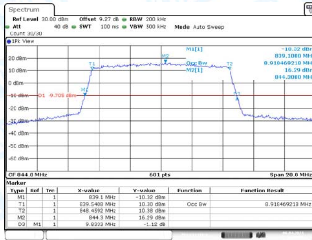
Band5-10MHz-16QAM-20600-50RB#0
