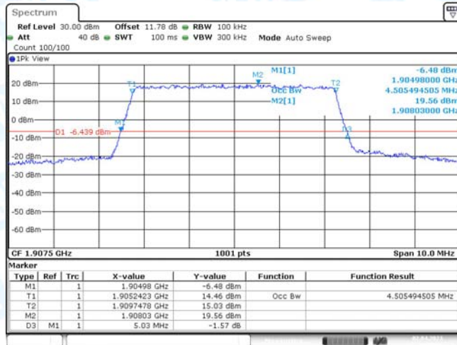
Band2-5MHz-QPSK-19175-25RB#0
