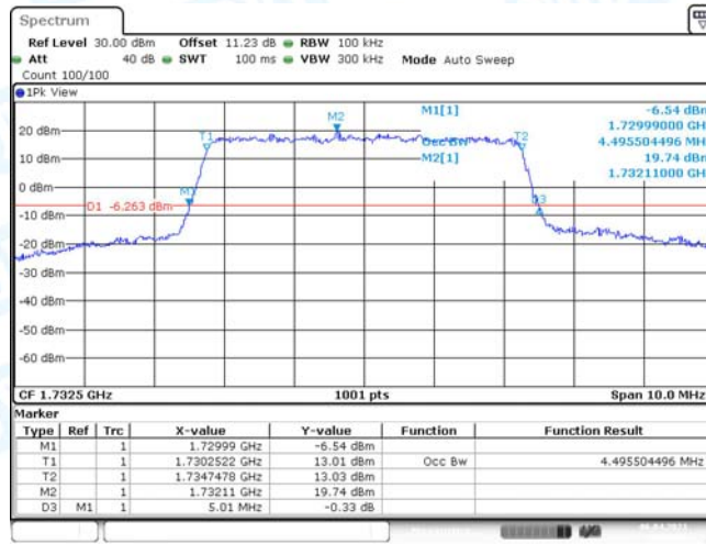
Band4-5MHz-16QAM-20175-25RB#0
