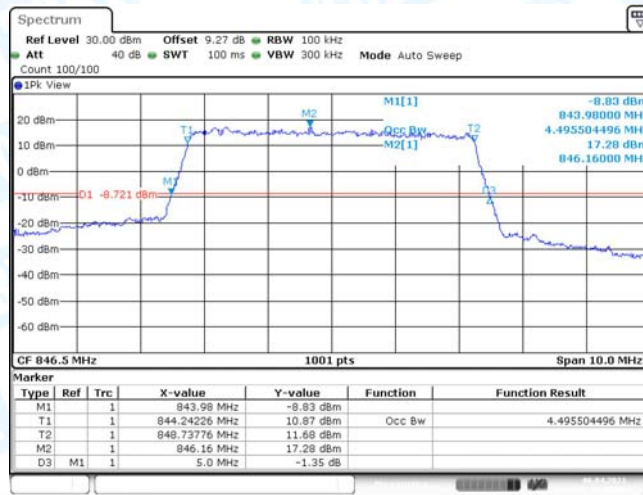
Band5-5MHz-QPSK-20625-25RB#0
