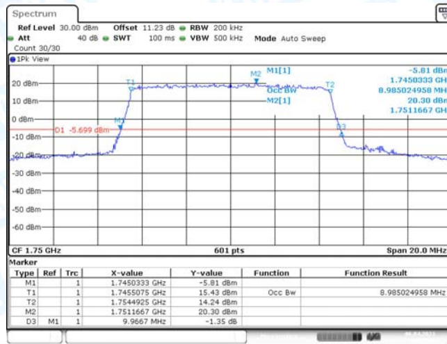
Band4-10MHz-QPSK-20350-50RB#0
