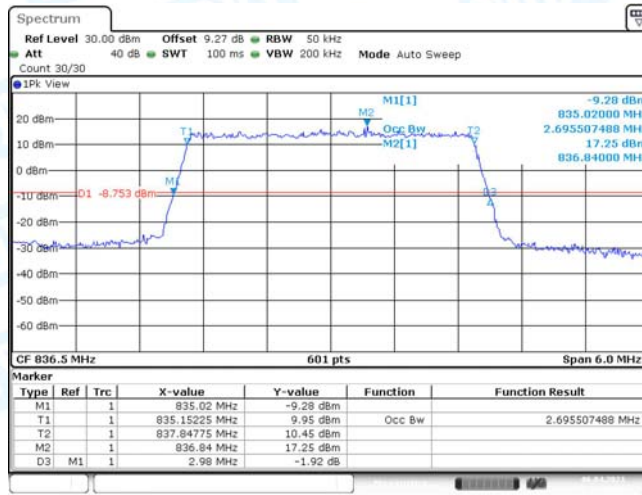
Band5-3MHz-QPSK-20525-15RB#0
