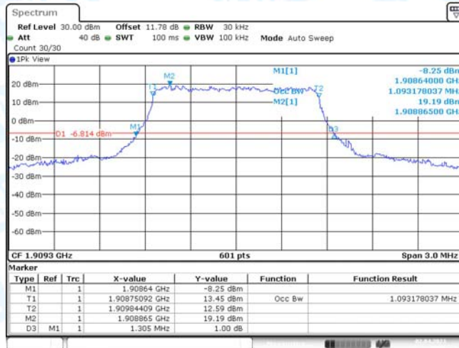
Band2-1.4MHz-16QAM-19193-6RB#0
