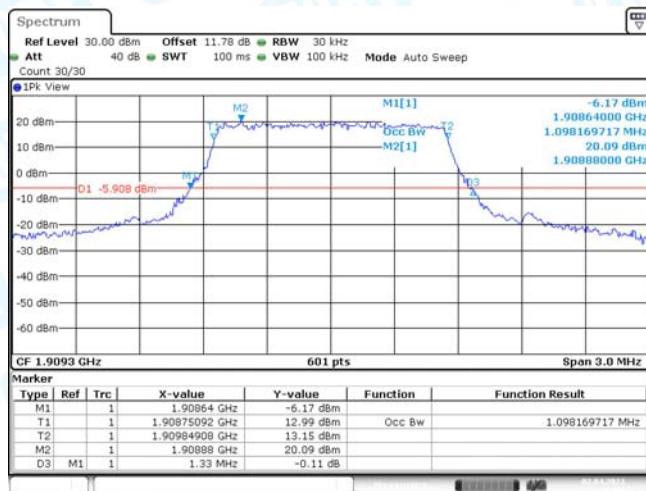
Band2-1.4MHz-QPSK-19193-6RB#0
