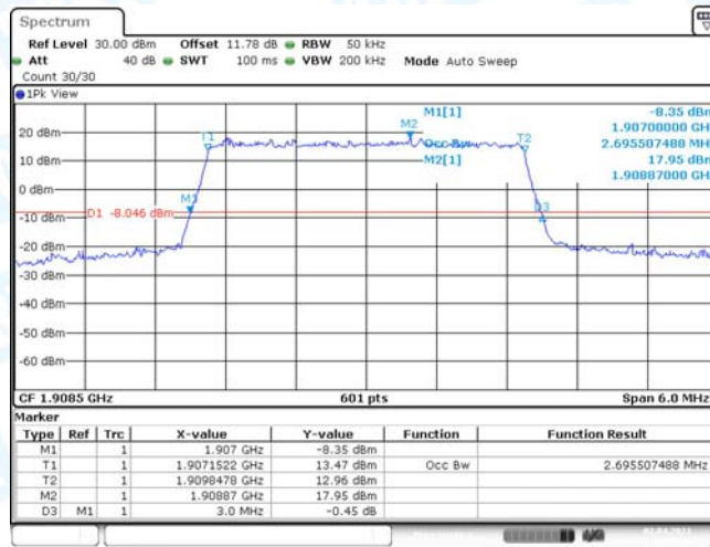
Band2-3MHz-16QAM-19185-15RB#0
