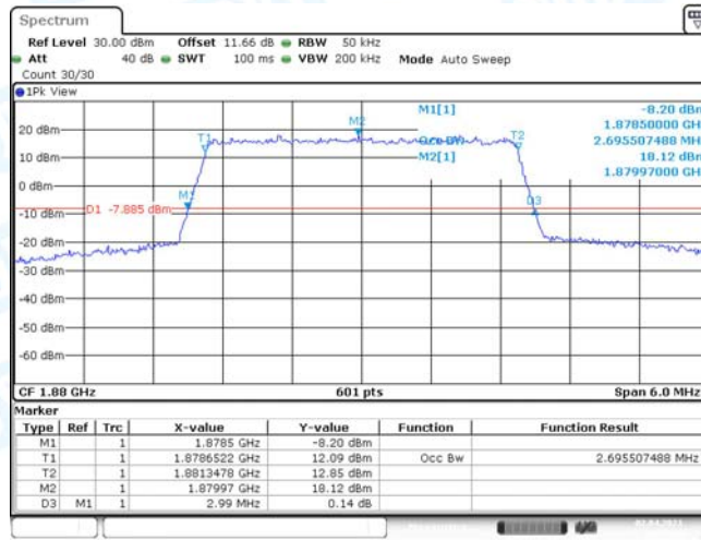
Band2-3MHz-16QAM-18900-15RB#0
