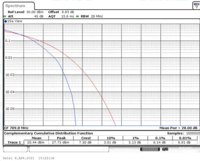
Band17-10MHz-16QAM-23790-1RB#0
