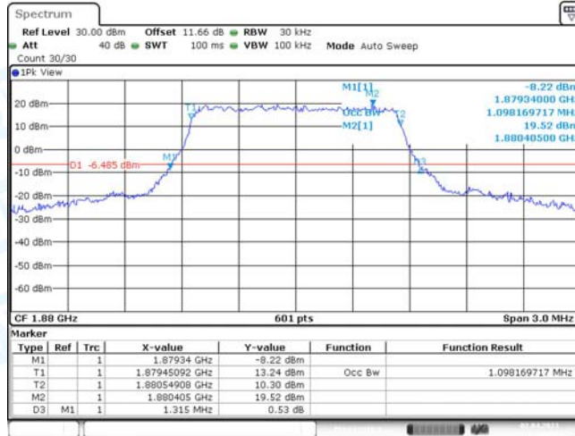
Band2-1.4MHz-16QAM-18900-6RB#0
