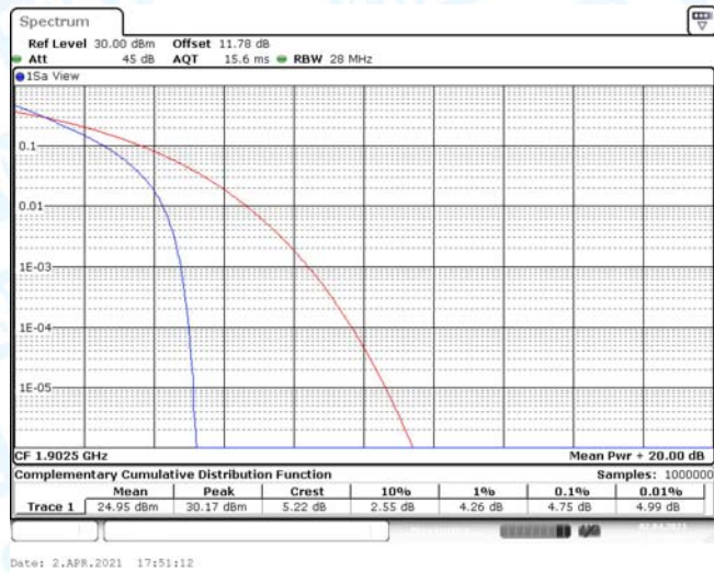
Band2-15MHz-16QAM-18675-1RB#0
