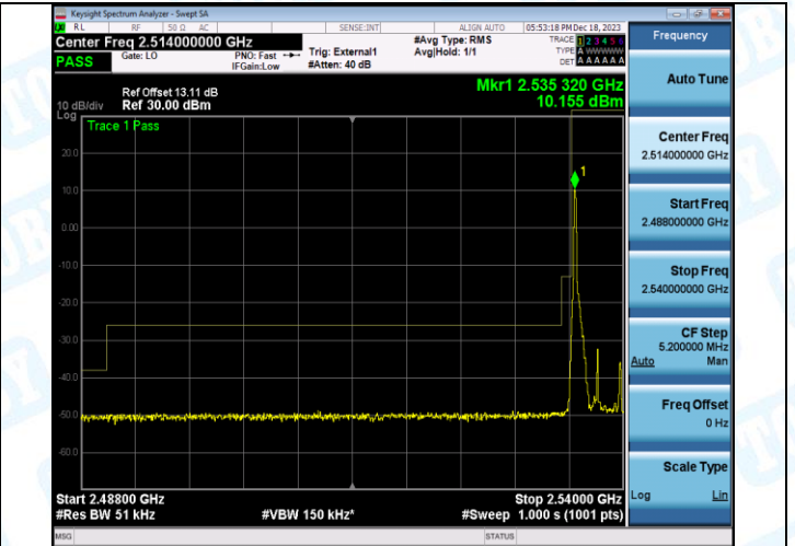
Band41_5MHz_16QAM_40065_1RB#24
