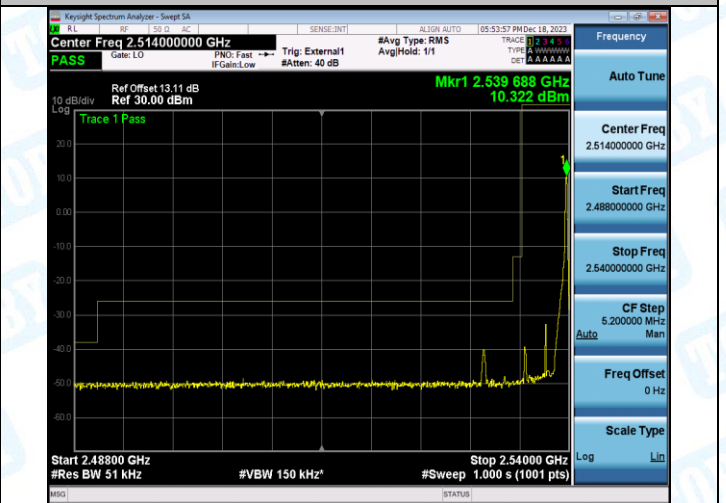
Band41_5MHz_16QAM_40065_25RB#0
