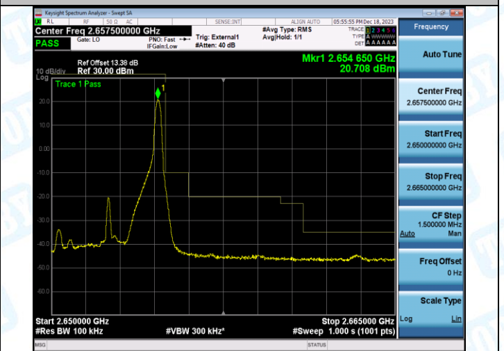
Band41_5MHz_16QAM_41215_25RB#0
