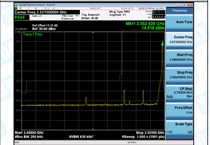
Band41_20MHz_16QAM_40140_100RB#0
