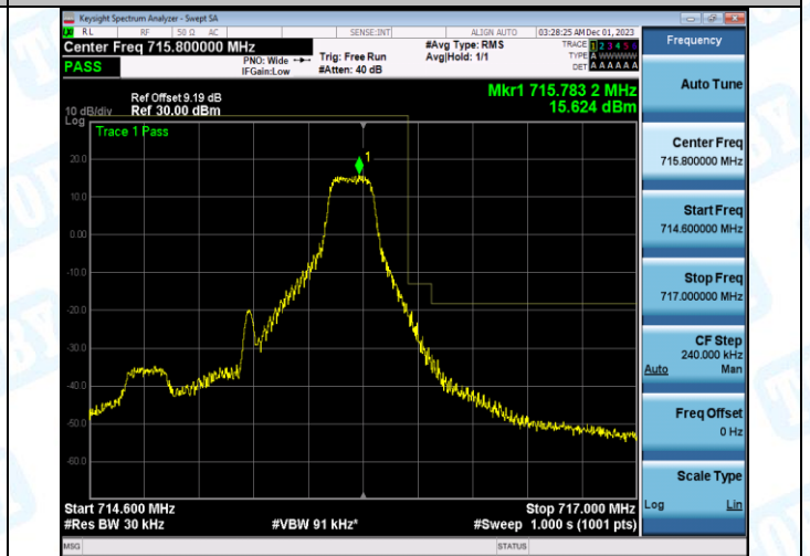
Band12_1.4MHz_16QAM_23173_6RB#0
