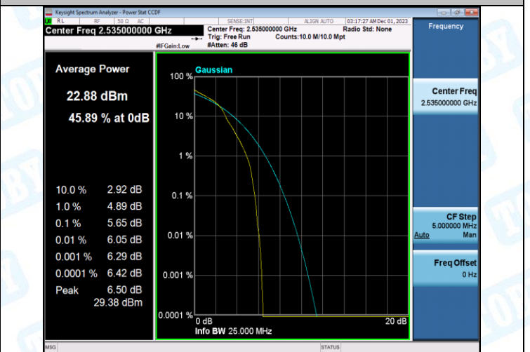
Band7-20MHz-16QAM-21100-100RB#0-PASS
