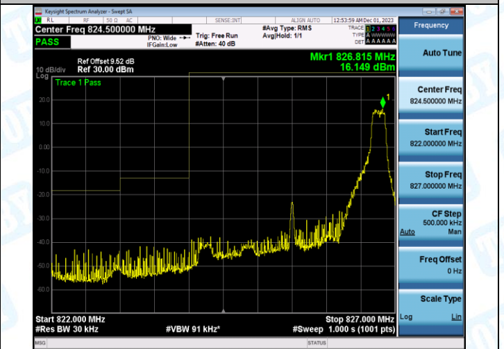
Band5_3MHz_16QAM_20415_15RB#0
