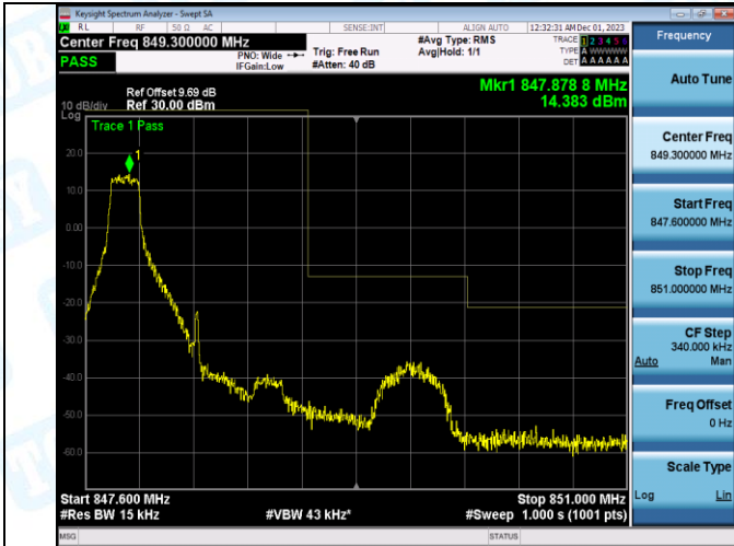
Band5_1.4MHz_QPSK_20643_1RB#5
