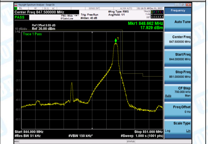
Band5_5MHz_16QAM_20625_25RB#0
