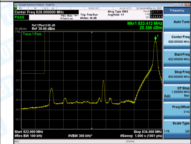
Band5_10MHz_16QAM_20450_50RB#0
