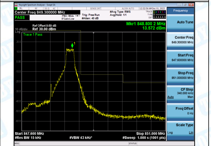
Band5_1.4MHz_16QAM_20643_6RB#0
