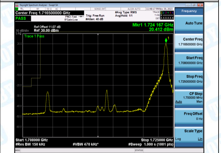
Band4_15MHz_16QAM_2025_75RB#0
