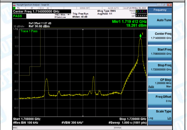
Band4_10MHz_16QAM_20000_50RB#0
