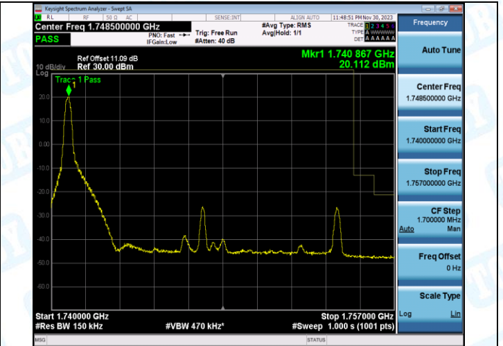
Band4_15MHz_16QAM_20325_1RB#74
