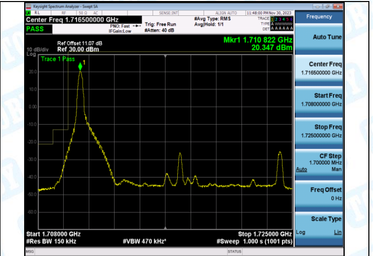
Band4_15MHz_16QAM_2025_1RB#74
