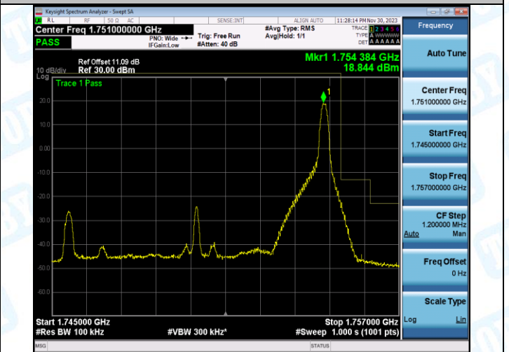
Band4_10MHz_16QAM_20350_50RB#0
