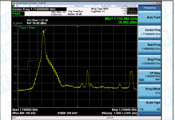
Band4_10MHz_16QAM_20000_1RB#49
