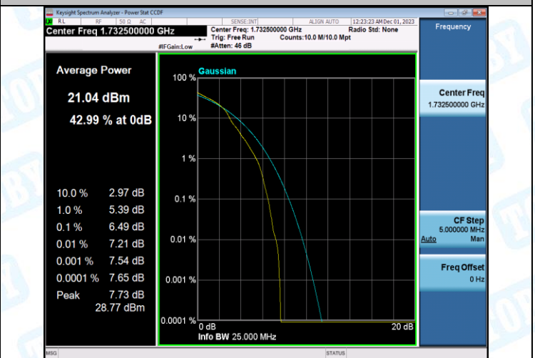
Band4-20MHz-16QAM-20175-100RB#0-PASS
