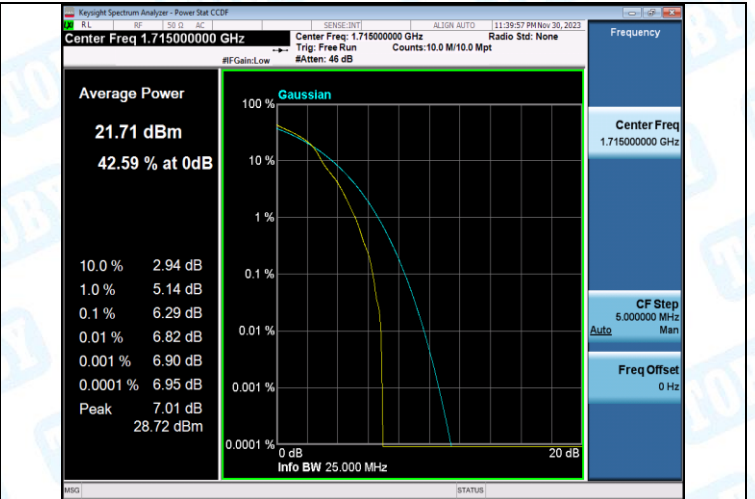
Band4-10MHz-16QAM-20000-50RB#0-PASS
