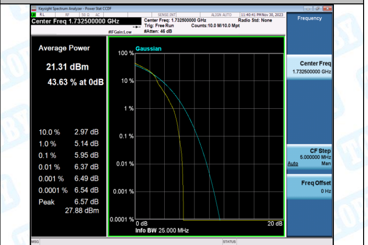
Band4-10MHz-16QAM-20175-50RB#0-PASS
