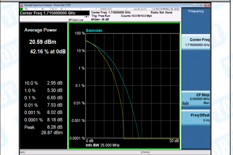
Band4-10MHz-16QAM-20175-1RB#0-PASS
