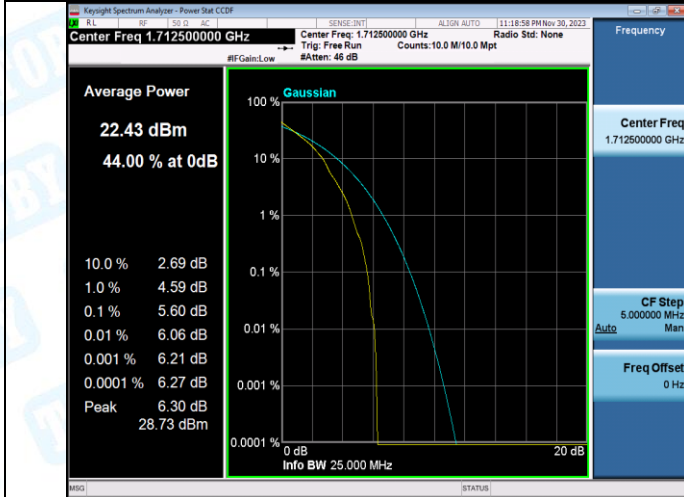
Band4-5MHz-QPSK-19975-25RB#0-PASS
