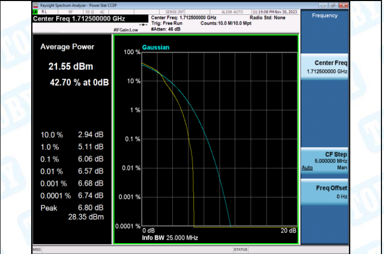
Band4-5MHz-16QAM-19975-25RB#0-PASS
