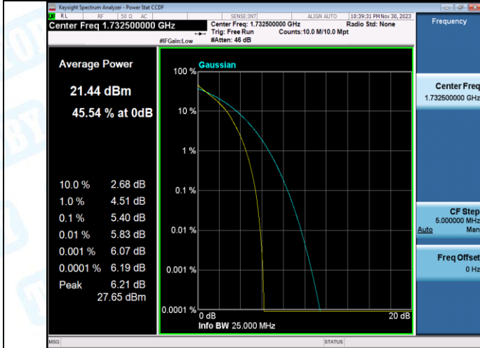
Band4-1.4MHz-QPSK-20393-1RB#0-PASS
