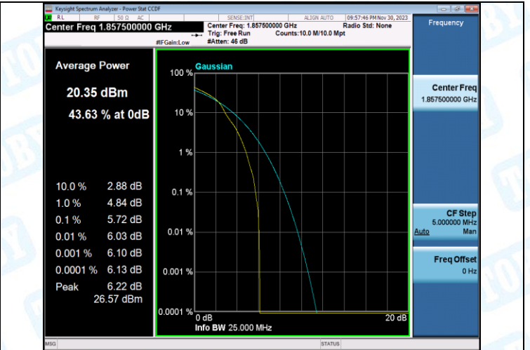
Band2-15MHz-16QAM-18675-75RB#0-PASS
