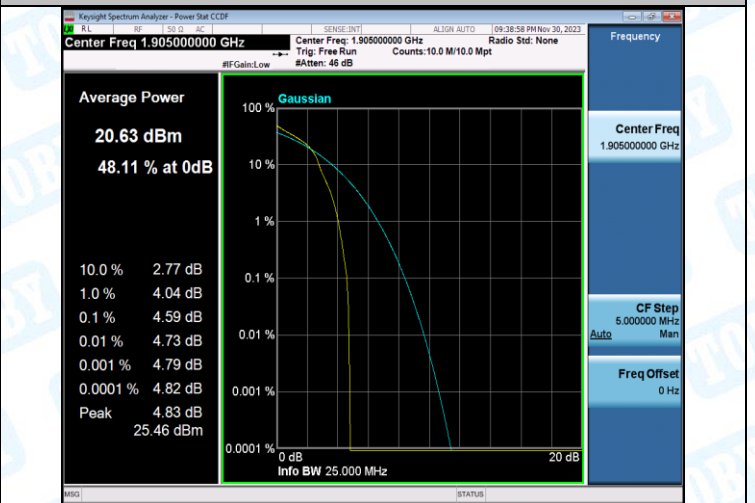
Band2-10MHz-16QAM-19150-50RB#0-PASS
