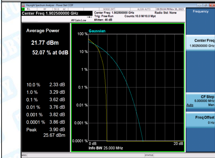
Band2-15MHz-QPSK-19125-75RB#0-PASS
