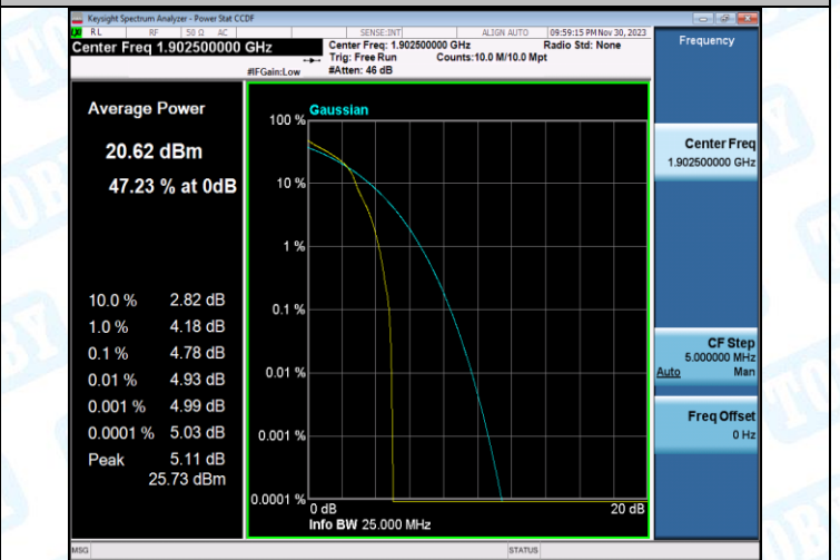
Band2-15MHz-16QAM-19125-75RB#0-PASS
