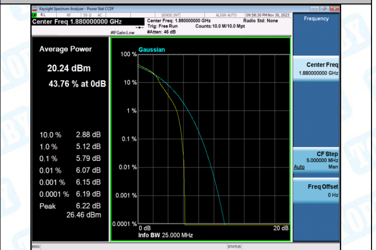
Band2-15MHz-16QAM-18900-75RB#0-PASS
