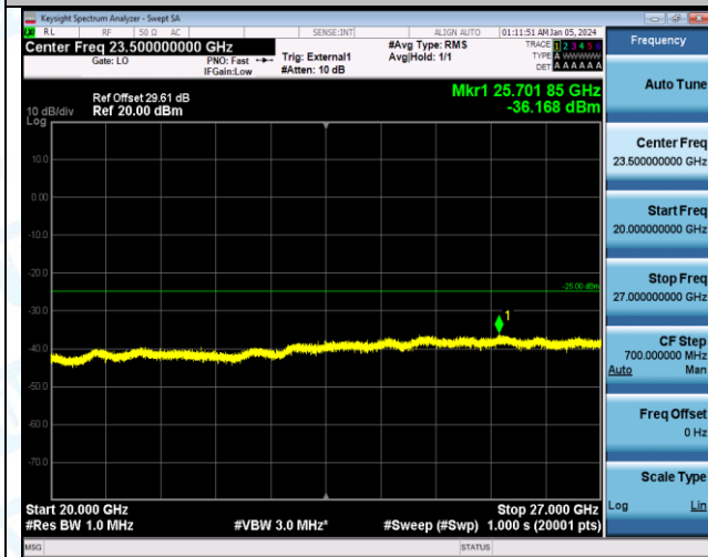
Band41_15MHz_16QAM_40590_1RB#0_30~1000_30~1000
