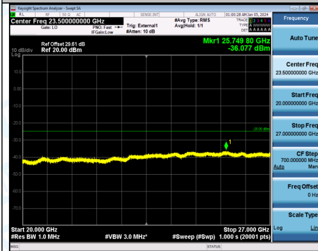
Band41_10MHz_16QAM_40590_1RB#0_30~1000_30~1000
