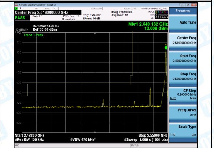
Band41_15MHz_16QAM_40115_75RB#0
