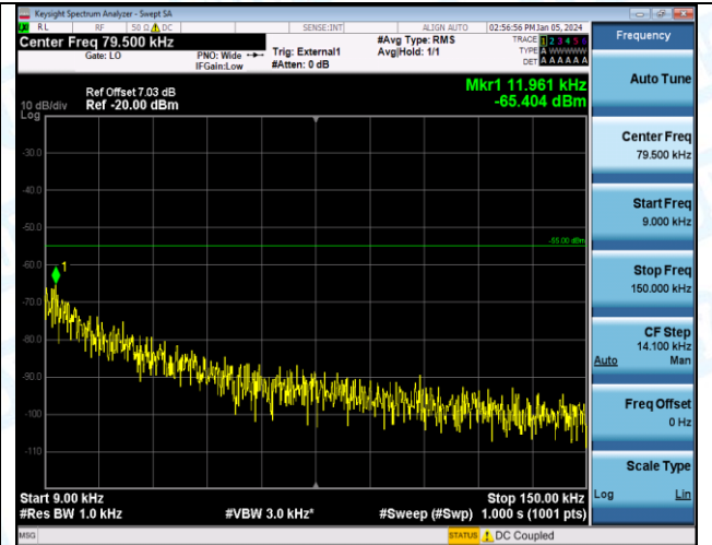
Band41_5MHz_16QAM_40065_1RB#0_20000~27000_20000~27000
