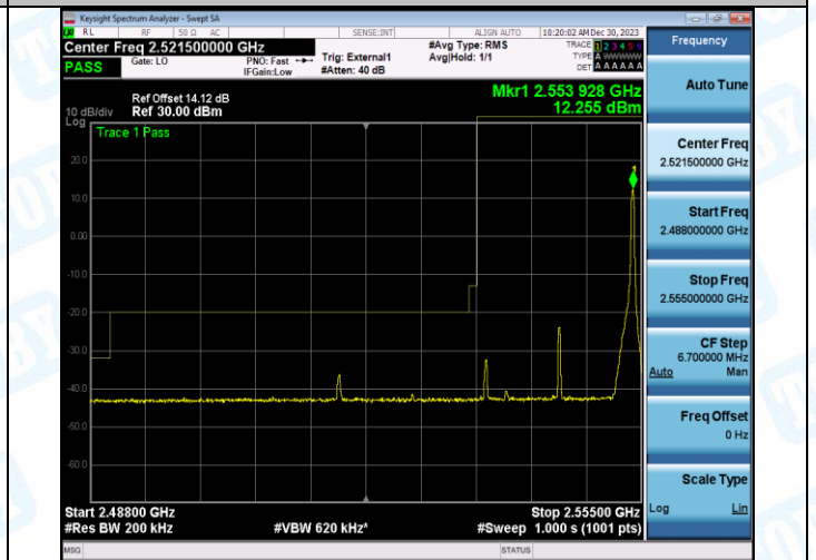
Band41_20MHz_16QAM_40140_100RB#0
