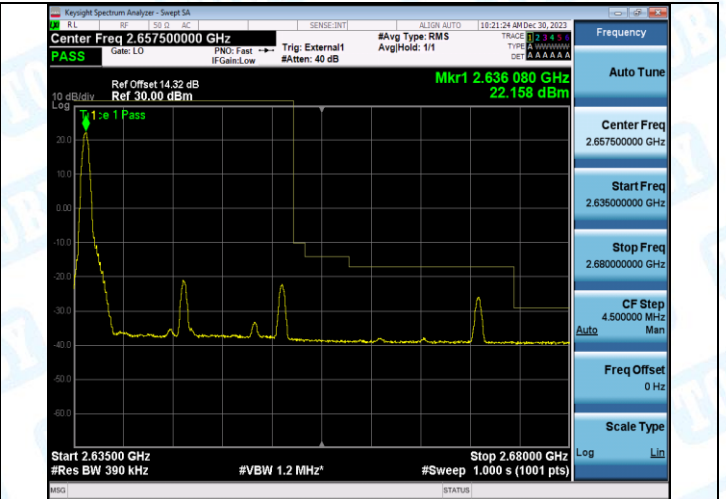
Band41_20MHz_16QAM_41140_1RB#99
