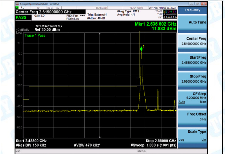
Band41_15MHz_16QAM_40115_1RB#74
