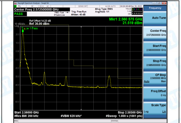
Band7_10MHz_16QAM_21400_1RB#49
