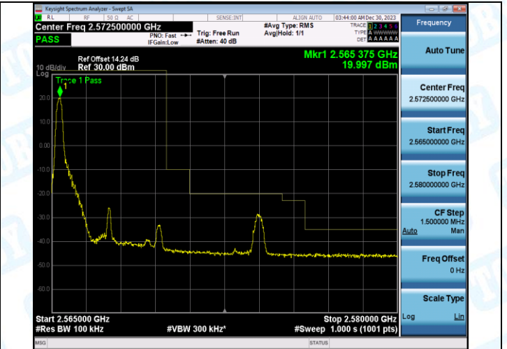
Band7_5MHz_16QAM_21425_1RB#24
