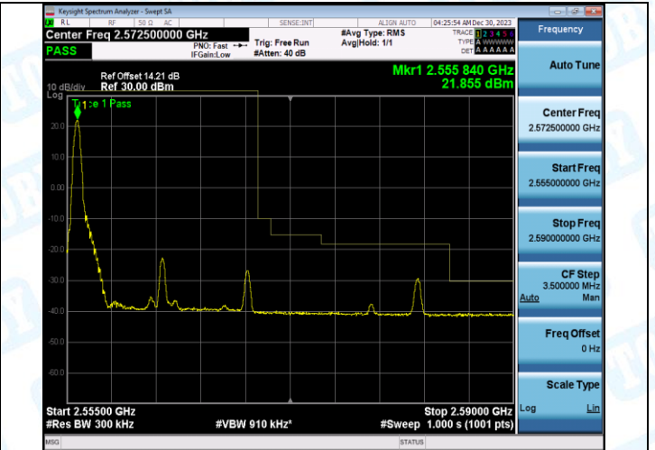
Band7_15MHz_16QAM_21375_1RB#74
