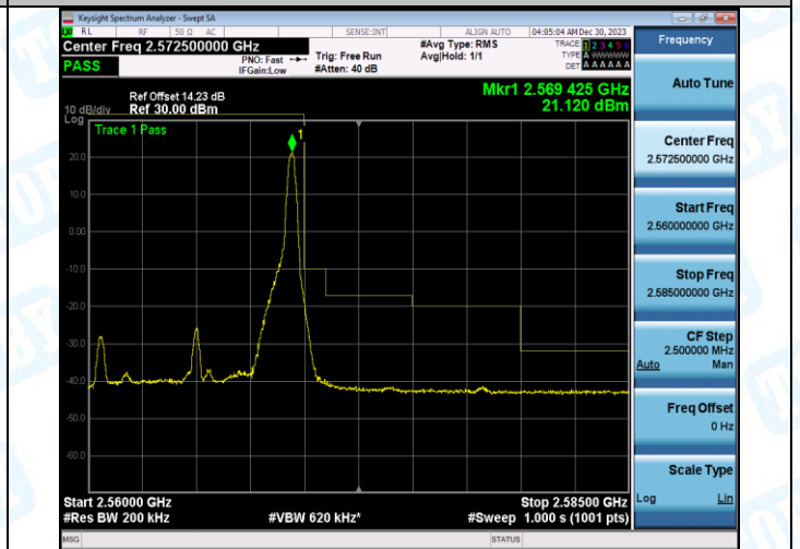
Band7_10MHz_16QAM_21400_50RB#0
