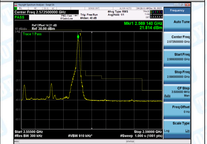
Band7_15MHz_16QAM_21375_75RB#0
