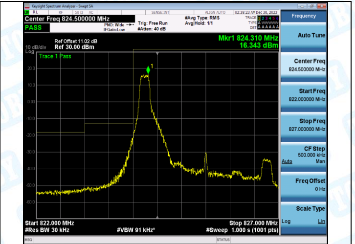
Band5_3MHz_16QAM_20415_1RB#14
