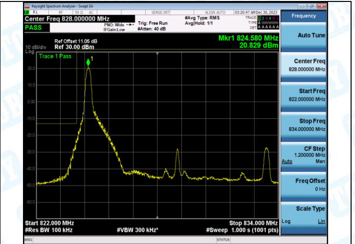
Band5_10MHz_16QAM_20450_1RB#49
