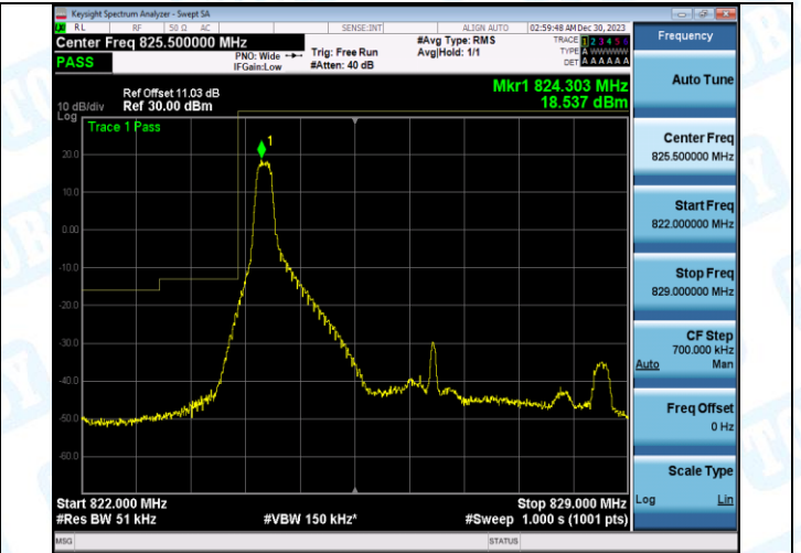
Band5_5MHz_16QAM_20425_1RB#24
