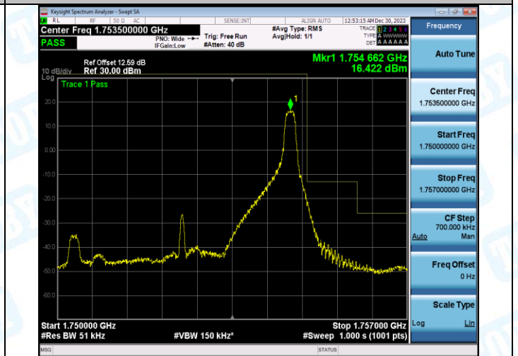
Band4_5MHz_16QAM_20375_25RB#0
