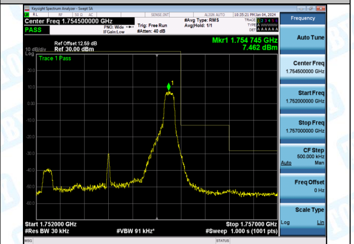
Band4_3MHz_QPSK_20385_15RB#0
