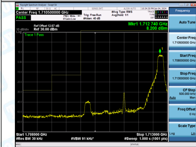
Band3_3MHz_QPSK_19965_15RB#0
