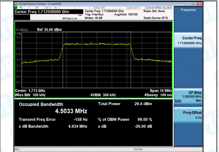
Band4-5MHz-16QAM-20175-25RB#0-PASS
