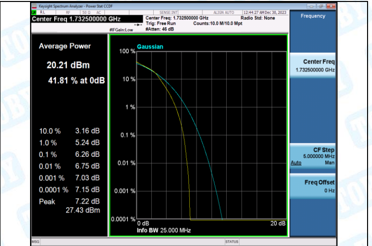
Band4-3MHz-16QAM-20385-1RB#0-PASS
