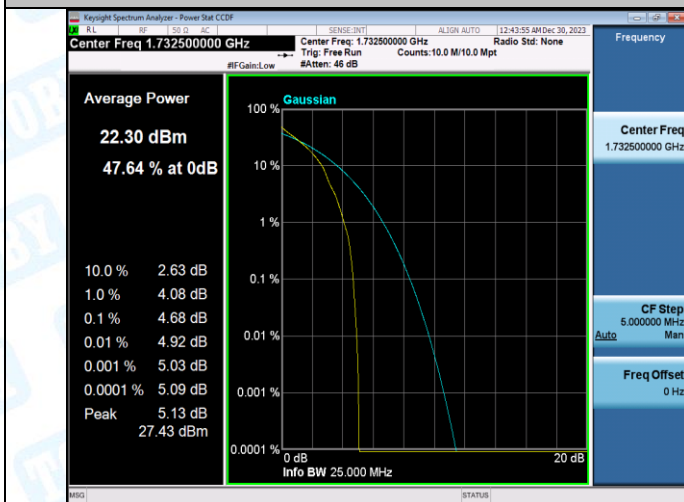
Band4-3MHz-QPSK-20175-15RB#0-PASS
