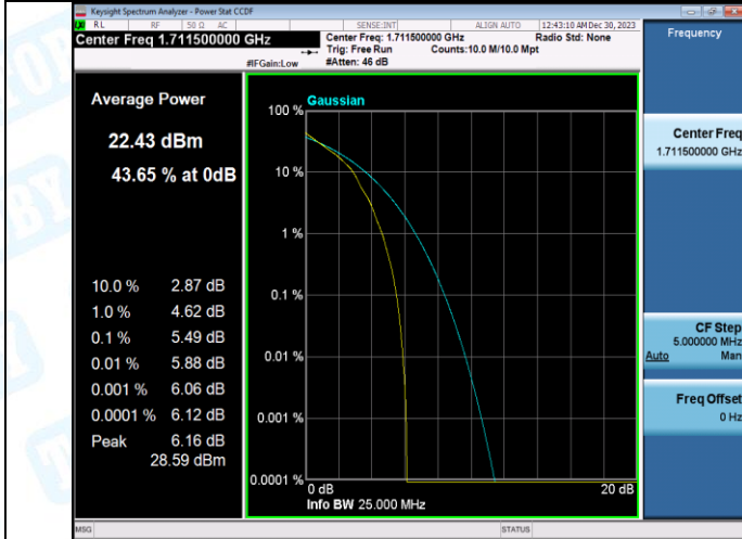
Band4-3MHz-QPSK-19965-15RB#0-PASS
