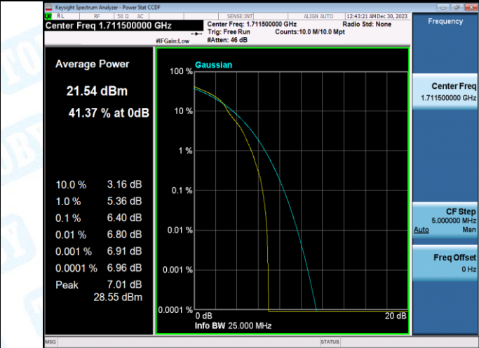
Band4-3MHz-16QAM-19965-15RB#0-PASS
