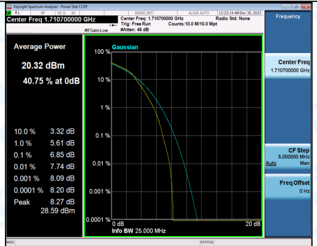
Band4-1.4MHz-16QAM-20175-1RB#0-PASS
