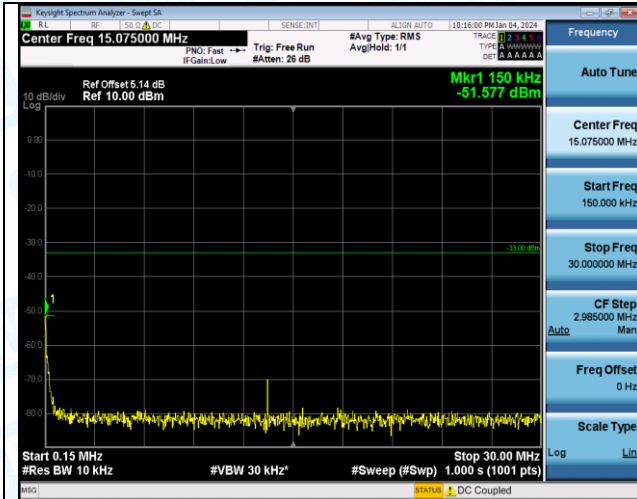
Band2_15MHz_QPSK_18675_1RB#0_1000-3000_1000-3000
