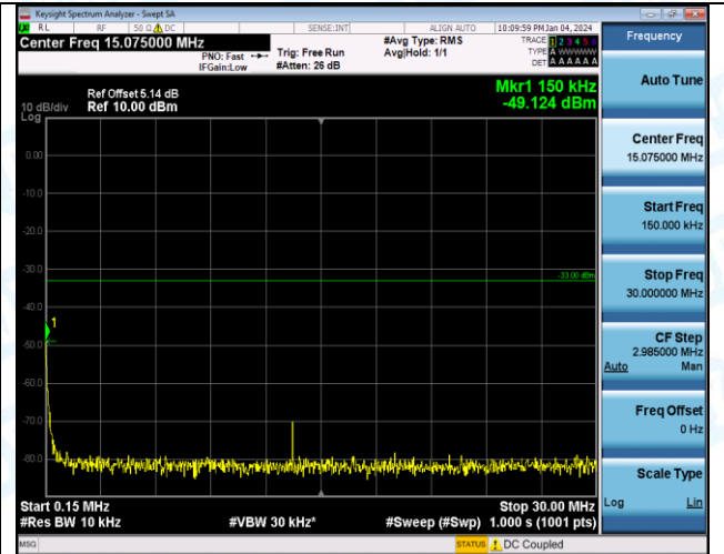
Band2_10MHz_QPSK_18650_1RB#0_1000~3000_1000~3000
