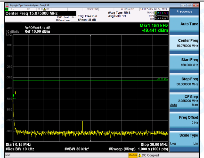
Band2_10MHz_16QAM_18900_1RB#0_1000~3000_1000~3000
