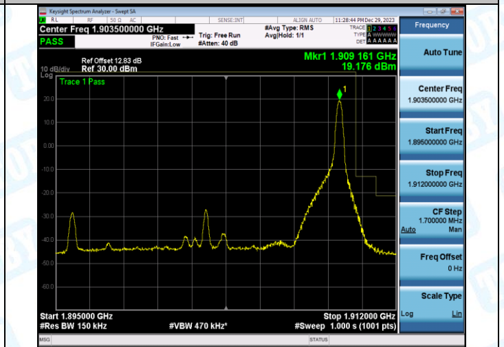
Band2_15MHz_16QAM_19125_75RB#0
