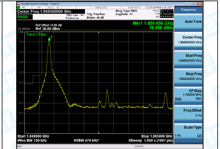
Band2_15MHz_16QAM_18675_1RB#74
