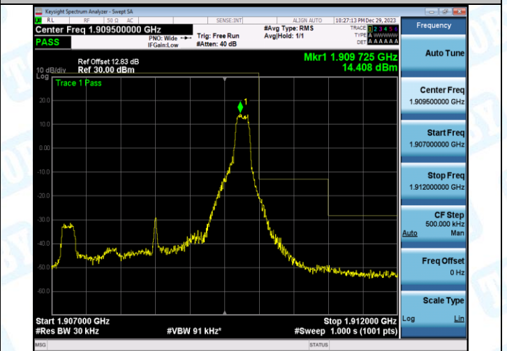
Band2_3MHz_16QAM_19185_15RB#0
