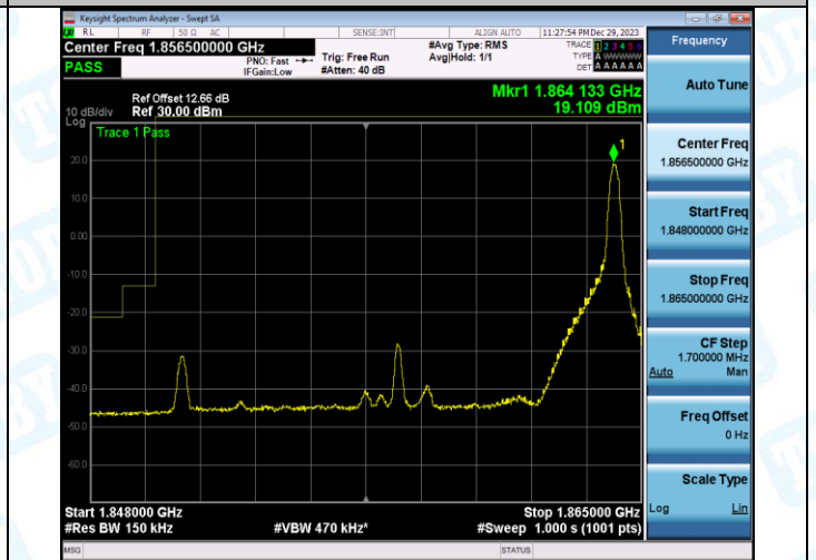
Band2_15MHz_16QAM_18675_75RB#0
