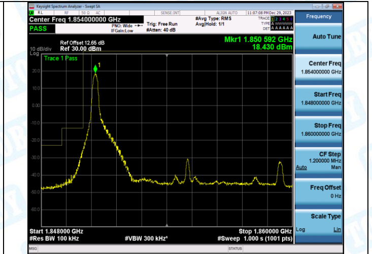
Band2_10MHz_16QAM_18650_1RB#49
