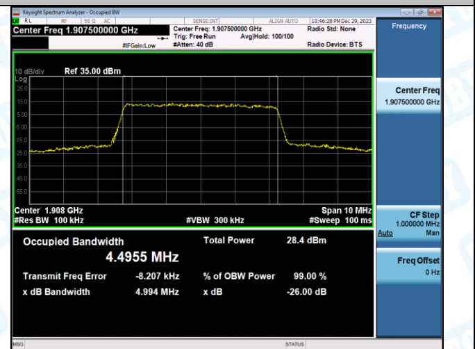
Band2-10MHz-16QAM-18650-50RB#0-PASS
