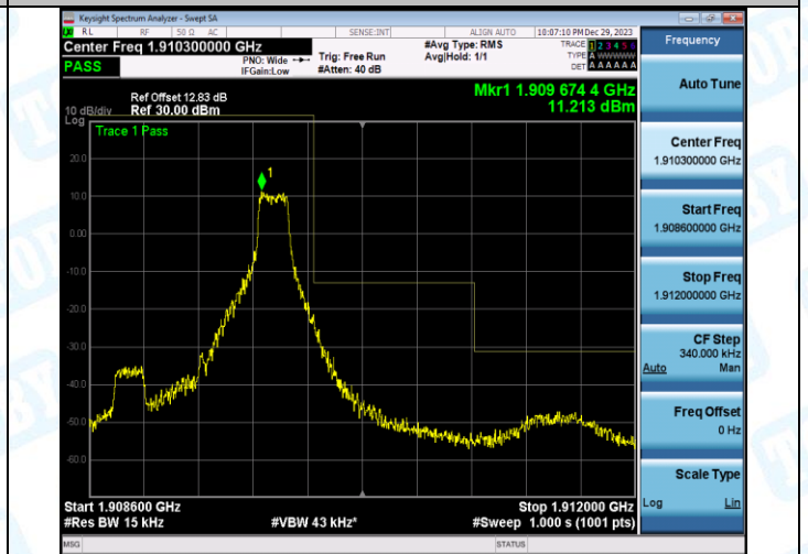
Band2_1.4MHz_16QAM_19193_6RB#0
