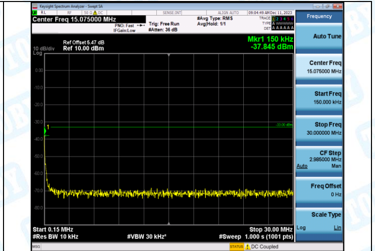
Band2-9400-5-0.15~30MHz-PASS
