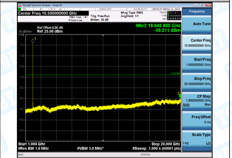
Band2-9262-5-1000~20000MHz-PASS
