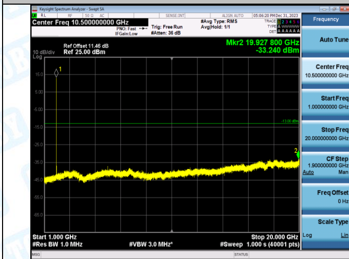
Band2-9538-2-10.500000000 GHz
