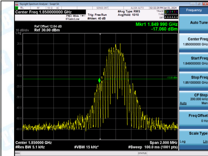
EGPRS1900-512-2-PASS
