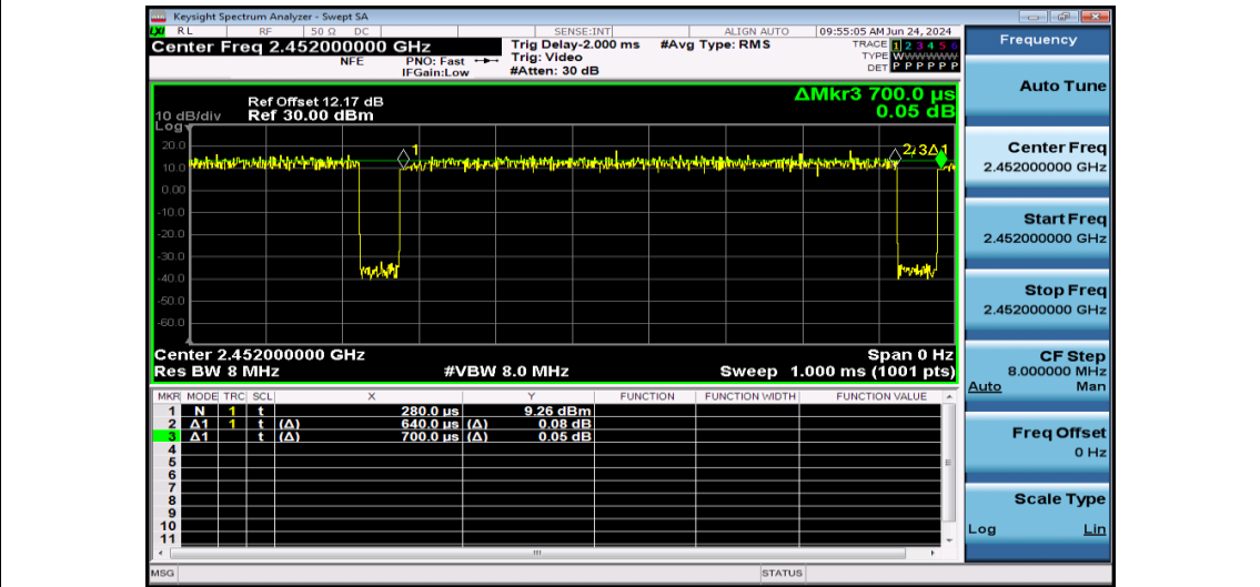
NTNV-11N40MIMO-Ant1-2452
