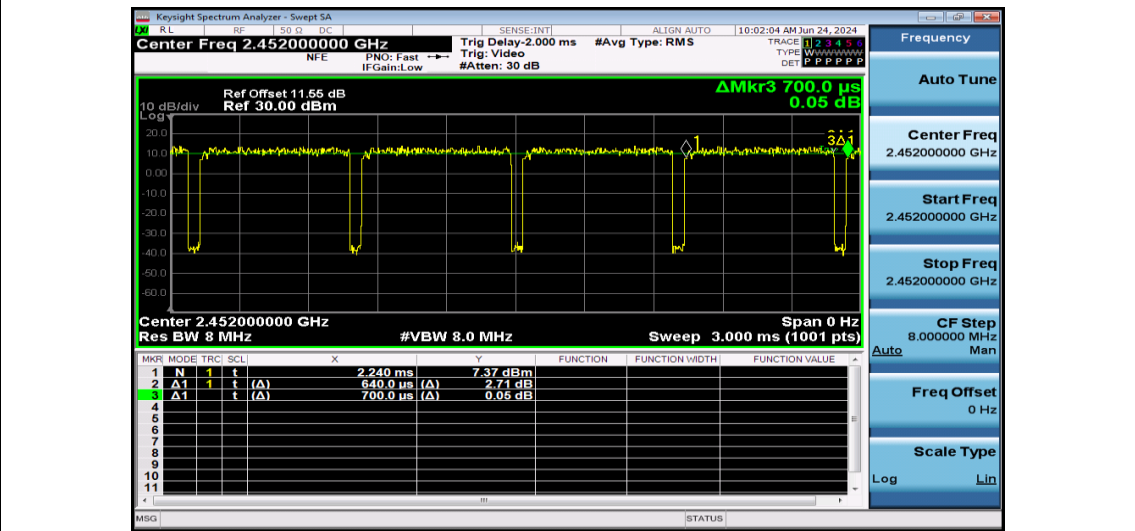
NTNV-11N40MIMO-Ant2-2452
