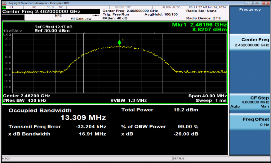
11B-Ant1-2462
