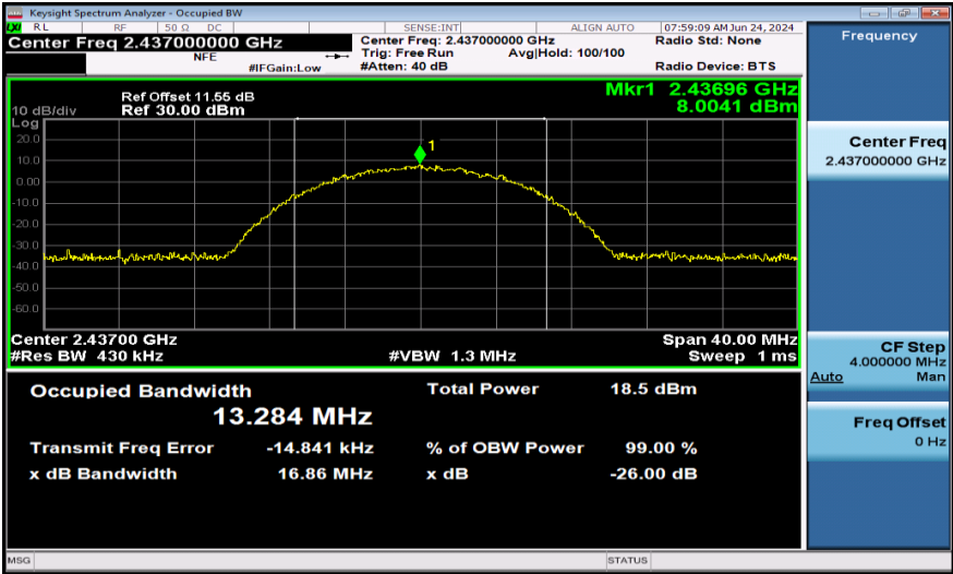
11B-Ant2-2437
