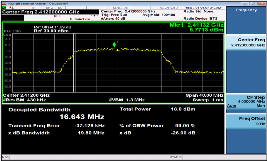
11G-Ant2-2412
