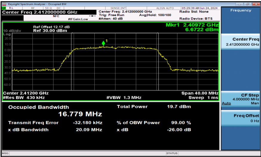
11G-Ant1-2412
