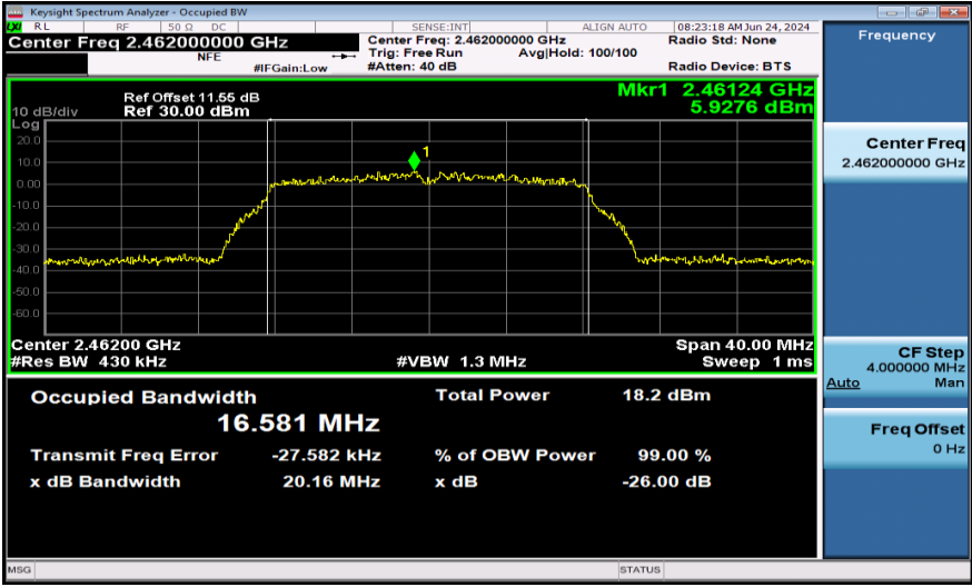
11G-Ant2-2462
