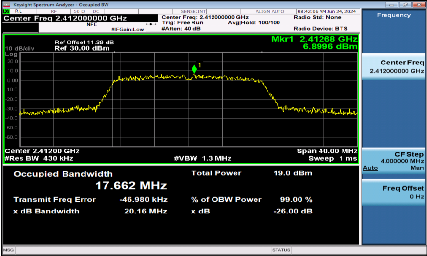
11N20MIMO-Ant2-2412
