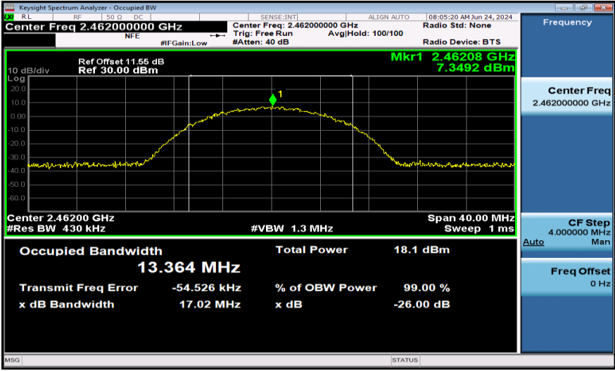
11B-Ant2-2462
