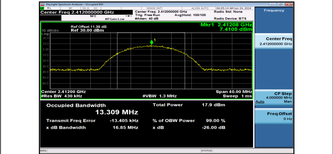
11B-Ant2-2412
