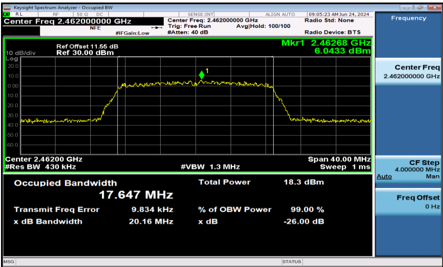
11N20MIMO-Ant2-2462
