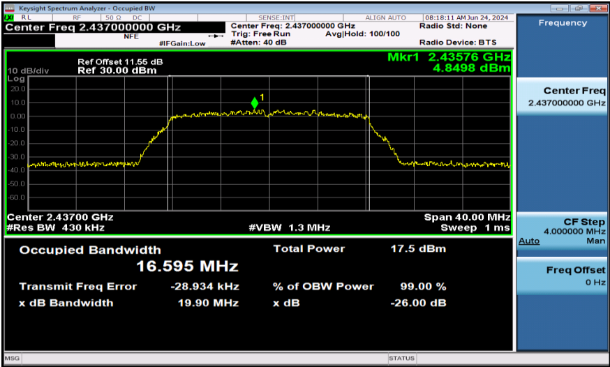
11G-Ant2-2437
