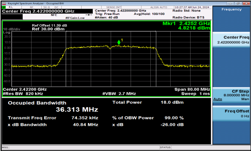
11N40MIMO-Ant2-2422
