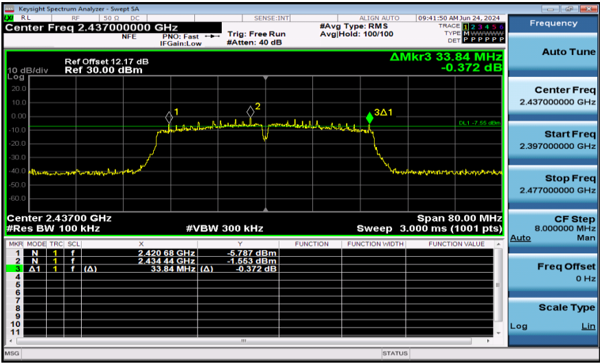
11N40MIMO-Ant1-2437-PASS
