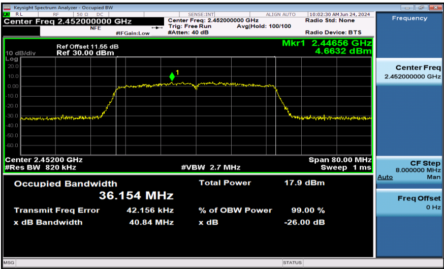
11N40MIMO-Ant2-2452
