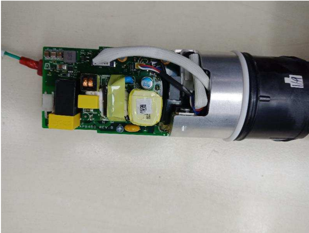
Power Board of Chicony version
