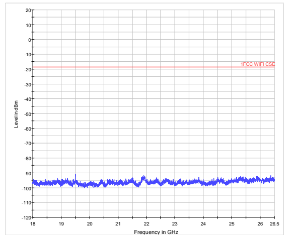
802.11b CH6 18GHz to 26.5GHz
