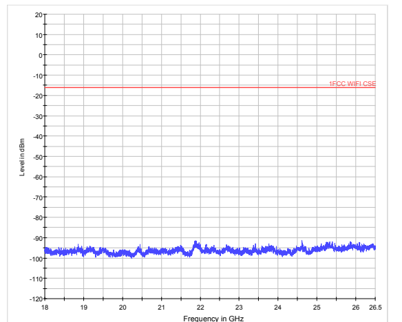
802.11b CH11 18GHz to 26.5GHz
