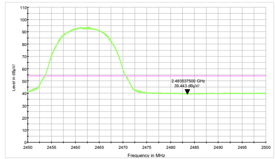
802.11g-Channel 11: Peak
