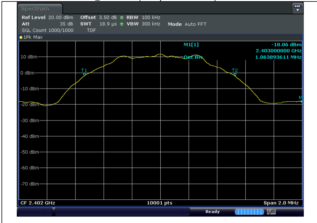
Test mode : Bluetooth LE_2 402 MHz(Occupied Bandwidth)
