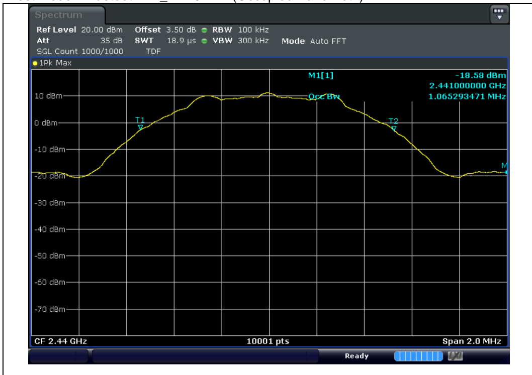
Test mode : Bluetooth LE_2 440 MHz(Occupied Bandwidth)
