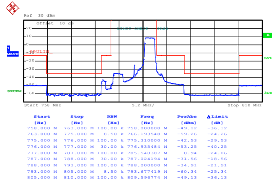
16QAM & RB Size 38
