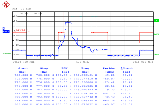
16QAM & RB Size 12
