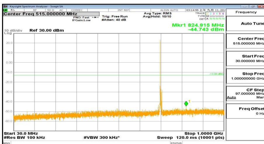
30MHz-1000MHz_FreqMid_BW(5MHz)_RB(1@0)_QPSK_Band12
