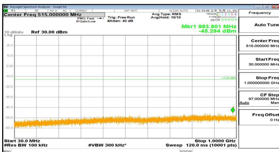
30MHz-1000MHz_FreqHigh_BW( 1D4MHz)_RB(1@5)_QPSK_Band25
