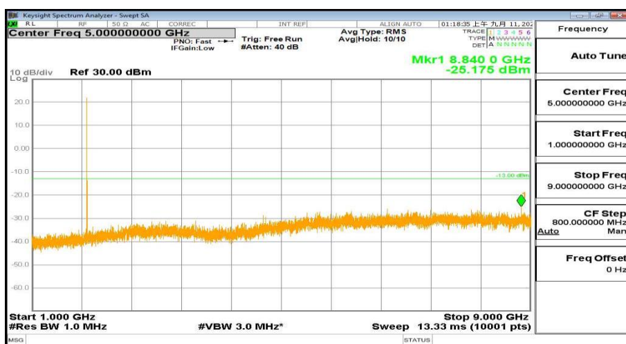
1000MHz-9000MHz_FreqMid_BW( 3MHz)_RB(1@0)_QPSK_Band25
