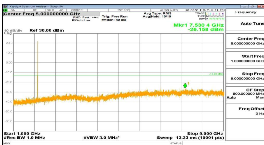
1000MHz-9000MHz_FreqHigh_BW( 3MHz)_RB(1@14)_QPSK_Band25
