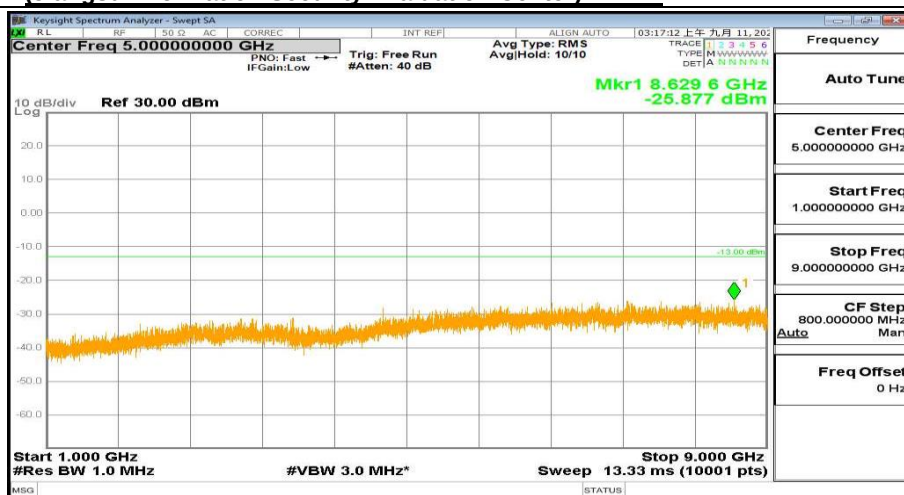
1000MHz-9000MHz_FreqMid_BW(3MHz)_RB(1@0)_QPSK_Band12
