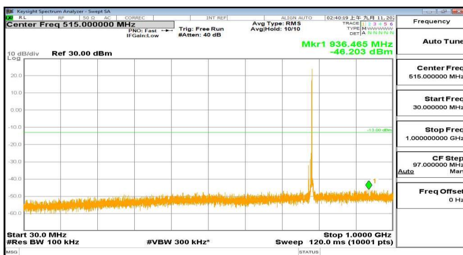
30MHz-1000MHz_FreqHigh_BW( 5MHz)_RB(1@24)_QPSK_Band13
