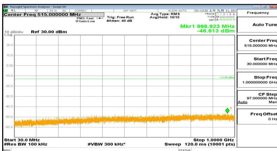
30MHz-1000MHz_FreqMid_BW( 1D4MHz)_RB(1@0)_QPSK_Band25
