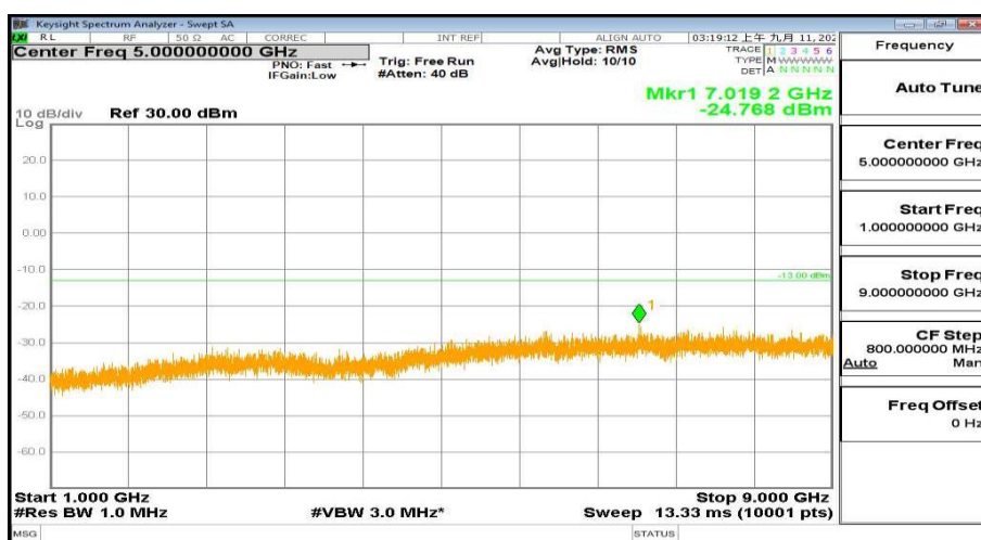
1000MHz-9000MHz_FreqMid_BW(10MHz)_RB(1@0)_QPSK_Band12
