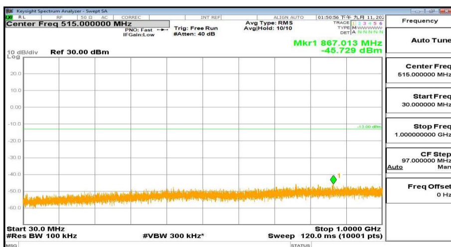
30MHz-1000MHz_FreqMid_BW(_1D4MHz)_RB(1@0)_QPSK_Band2
