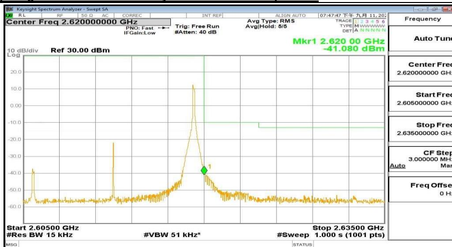
2605MHz-2635MHz_FreqHigh_BW( 15MHz)_RB(1@74)_QPSK_Band38
