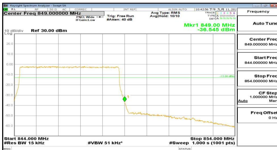
844MHz-854MHz_FreqHigh_BW(_5MHz)_RB(25@24)_QPSK_Band26
