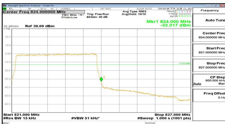
821MHz-827MHz_FreqHigh_BW(_3MHz)_RB(15@14)_QPSK_Band26
