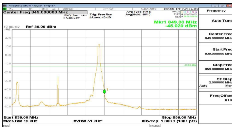
839MHz-859MHz_FreqHigh_BW(_10MHz)_RB(1@49)_QPSK_Band26
