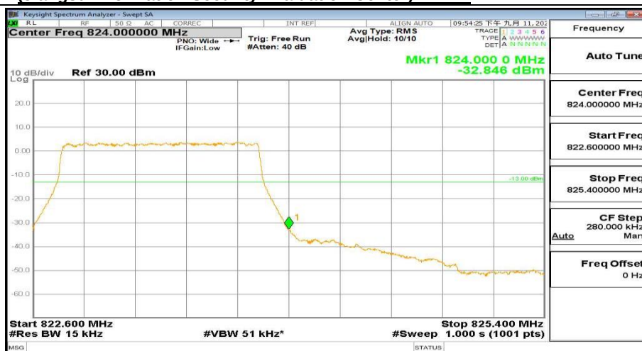
822.6MHz-825.4MHz_FreqHigh_BW(_1D4MHz)_RB(6@5)_QPSK_Band26
