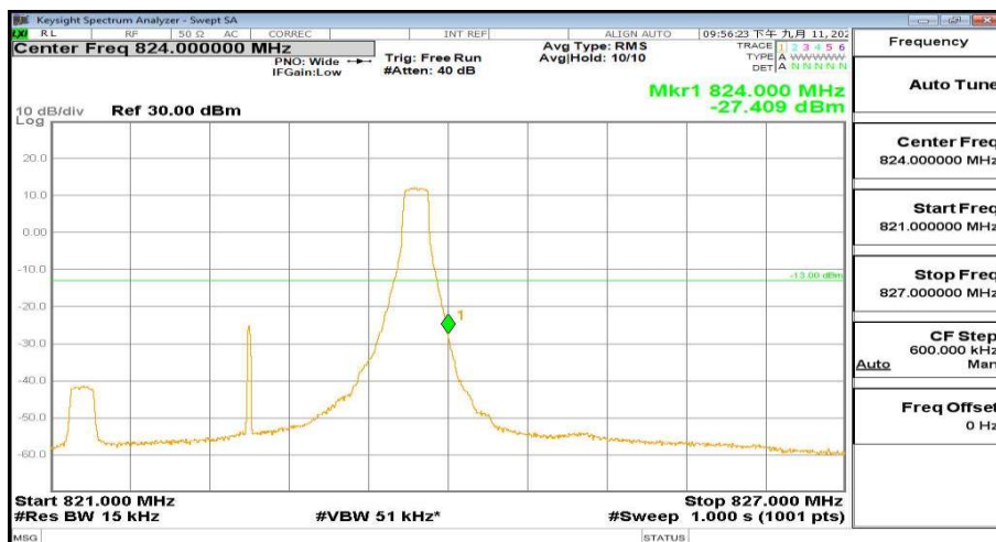
821MHz-827MHz_FreqHigh_BW(_3MHz)_RB(1@14)_QPSK_Band26
