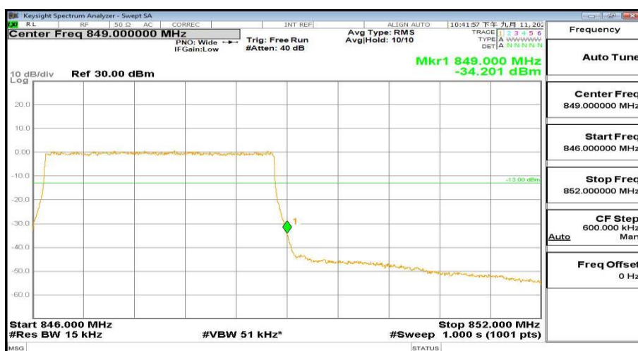
846MHz-852MHz_FreqHigh_BW(_3MHz)_RB(15@14)_QPSK_Band26
