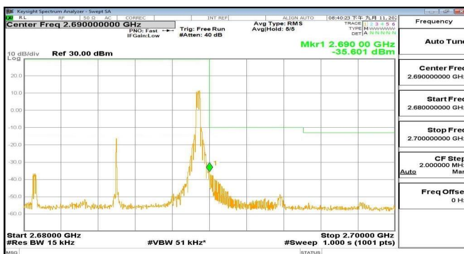
2680MHz-2700MHz_FreqHigh_BW(_10MHz)_RB(1@49)_QPSK_Band41
