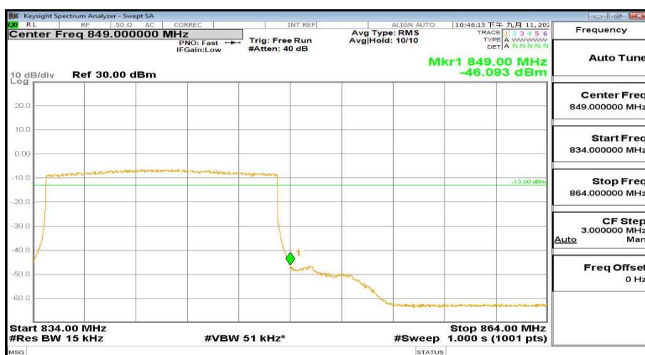
834MHz-864MHz_FreqHigh_BW( 15MHz)_RB(75@74)_QPSK_Band26
