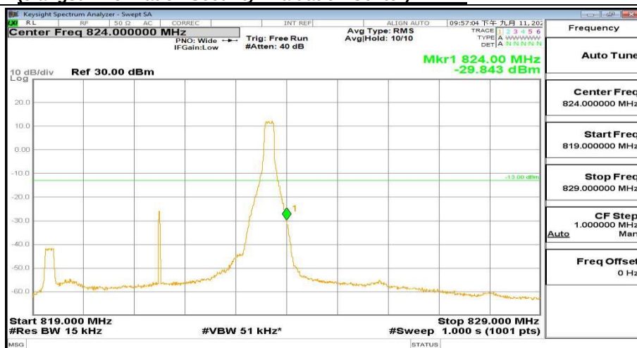
819MHz-829MHz_FreqHigh_BW(_5MHz)_RB(1@24)_QPSK_Band26
