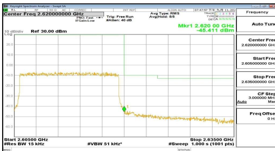
2605MHz-2635MHz_FreqHigh_BW( 15MHz)_RB(75@74)_QPSK_Band38
