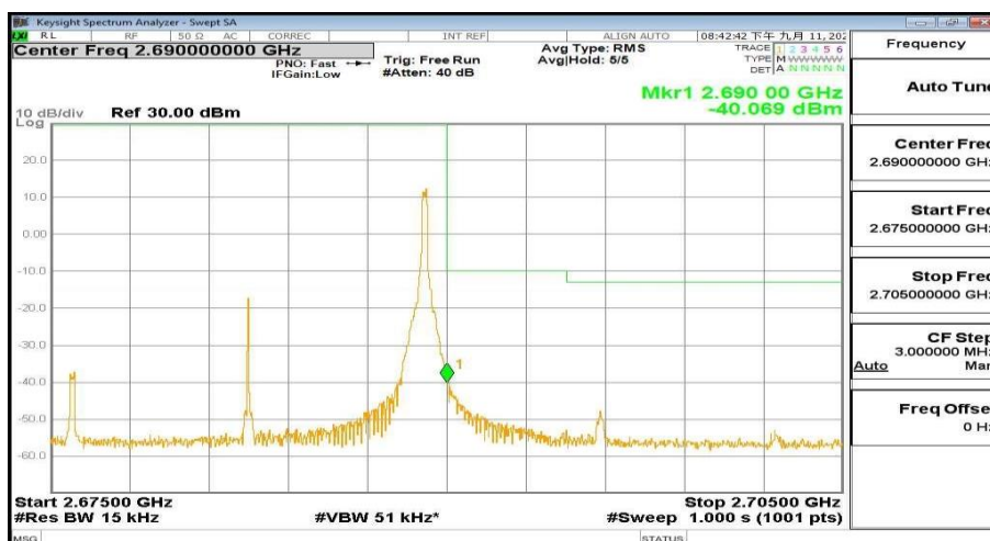
2675MHz-2705MHz_FreqHigh_BW(_15MHz)_RB(1@74)_QPSK_Band41
