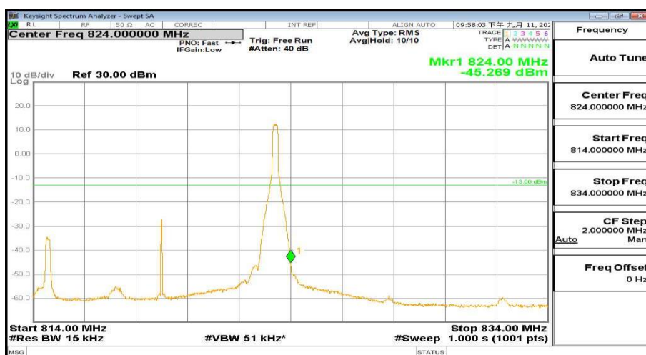
814MHz-834MHz_FreqHigh_BW(_10MHz)_RB(1@49)_QPSK_Band26
