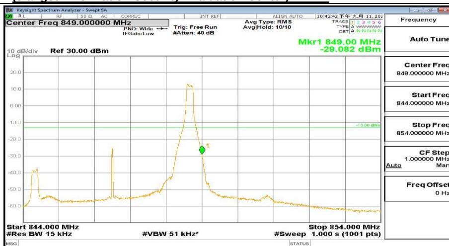
844MHz-854MHz_FreqHigh_BW(_5MHz)_RB(1@24)_QPSK_Band26
