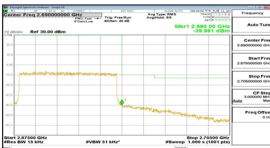
2675MHz-2705MHz_FreqHigh_BW(_15MHz)_RB(75@74)_QPSK_Band41
