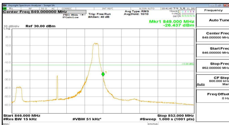
846MHz-852MHz_FreqHigh_BW(_3MHz)_RB(1@14)_QPSK_Band26
