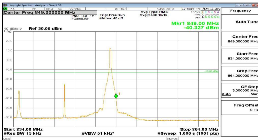
834MHz-864MHz_FreqHigh_BW( 15MHz)_RB(1@74)_QPSK_Band26
