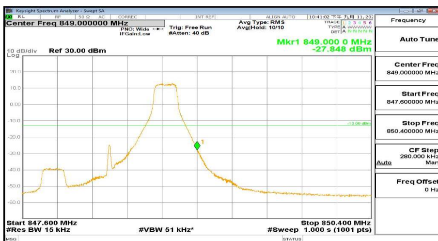
847.6MHz-850.4MHz_FreqHigh_BW(1D4MHz)_RB(1@5)_QPSK_Band26
