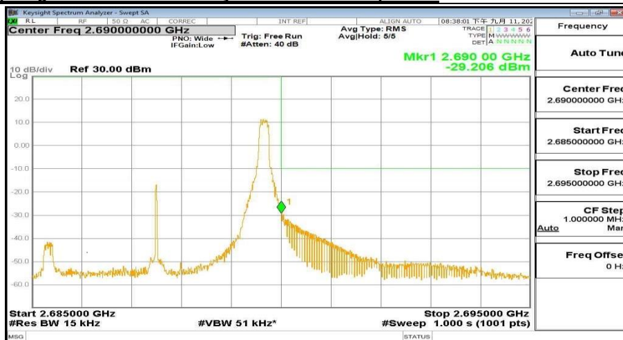
2685MHz-2695MHz_FreqHigh_BW(_5MHz)_RB(1@24)_QPSK_Band41
