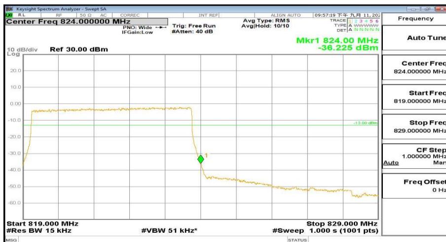
819MHz-829MHz_FreqHigh_BW(_5MHz)_RB(25@24)_QPSK_Band26
