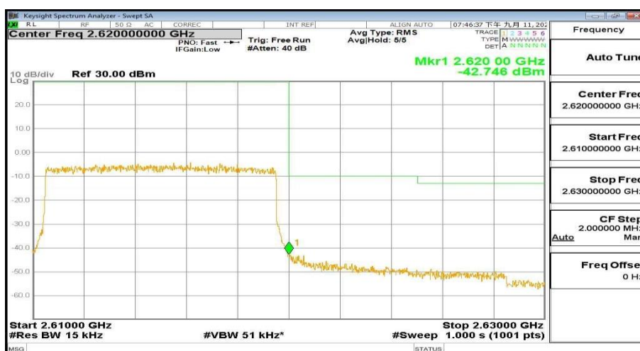
2610MHz-2630MHz_FreqHigh_BW( 10MHz)_RB(50@49)_QPSK_Band38
