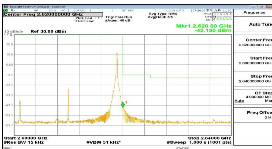
2600MHz-2640MHz_FreqHigh_BW( 20MHz)_RB(1@99)_QPSK_Band38
