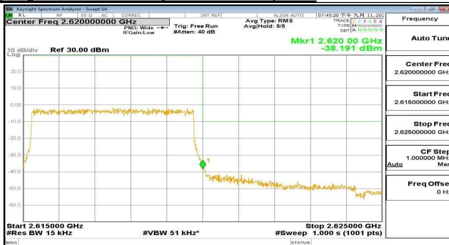
2615MHz-2625MHz_FreqHigh_BW( 5MHz)_RB(25@24)_QPSK_Band38
