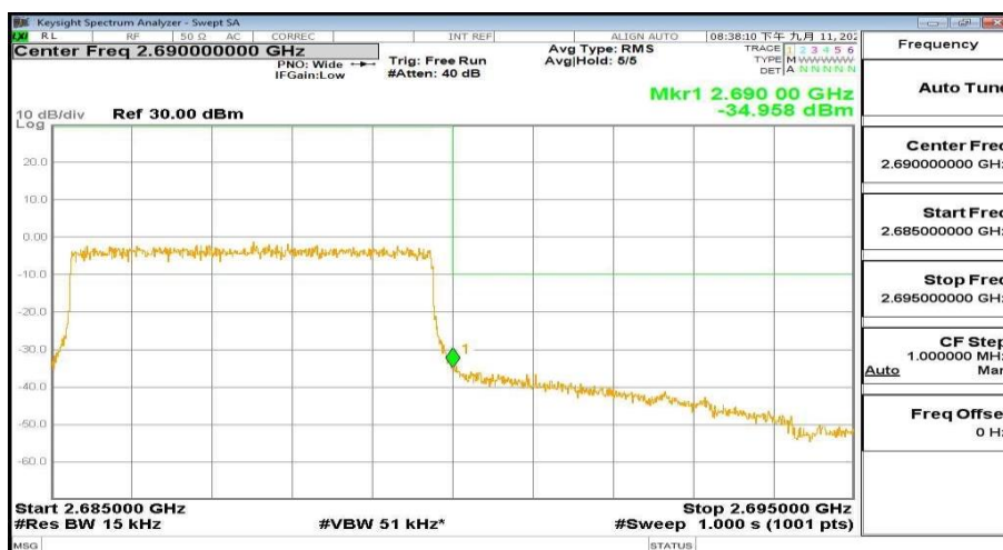
2685MHz-2695MHz_FreqHigh_BW(_5MHz)_RB(25@24)_QPSK_Band41
