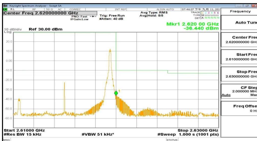
2610MHz-2630MHz_FreqHigh_BW( 10MHz)_RB(1@49)_QPSK_Band38
