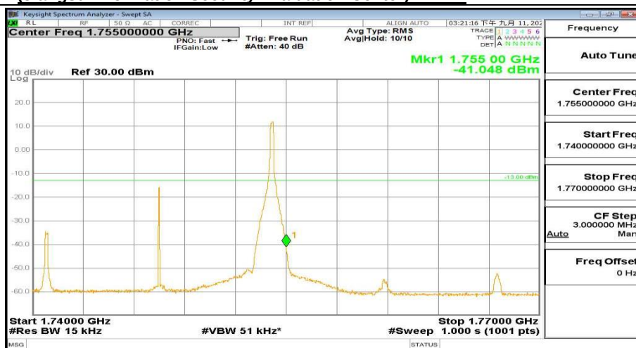
1740MHz-1770MHz_FreqHigh_BW(15MHz)_RB(1@74)_QPSK_Band4
