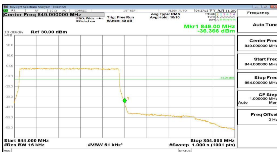
844MHz-854MHz_FreqHigh_BW(_5MHz)_RB(25@24)_QPSK_Band5
