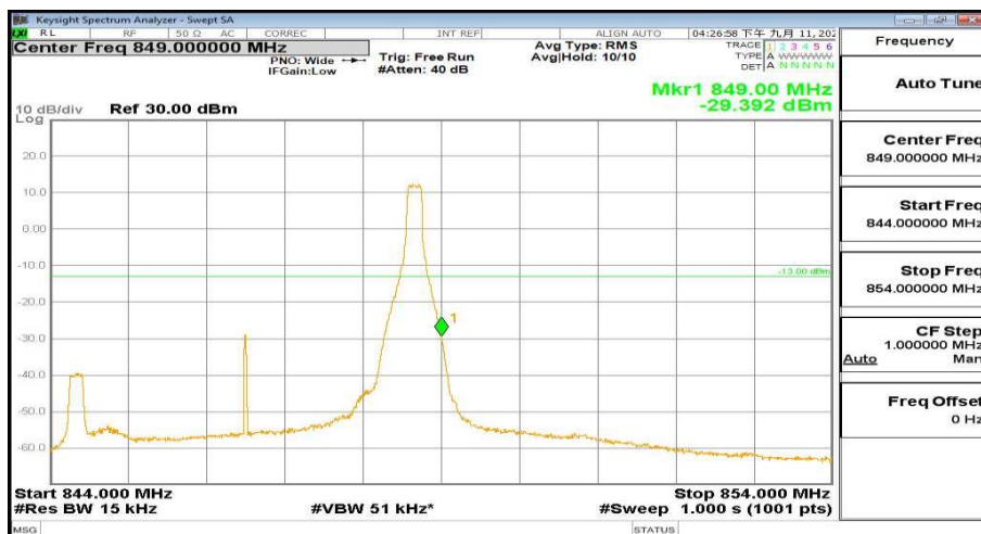
844MHz-854MHz_FreqHigh_BW(_5MHz)_RB(1@24)_QPSK_Band5
