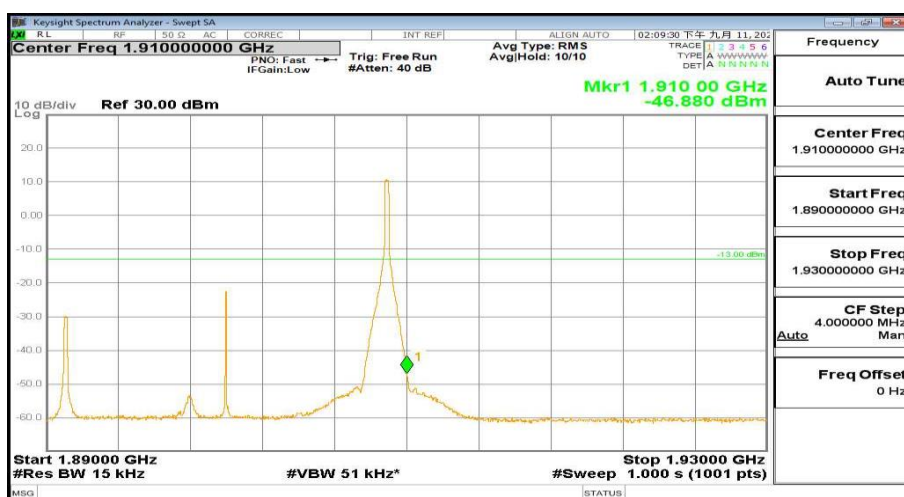
1890MHz-1930MHz_FreqHigh_BW(20MHz)_RB(1@99)_QPSK_Band2
