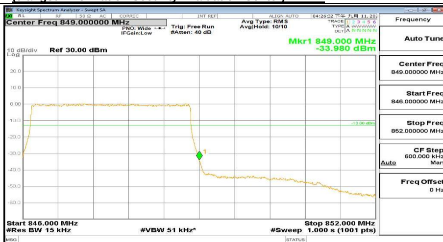
846MHz-852MHz_FreqHigh_BW(_3MHz)_RB(15@14)_QPSK_Band5
