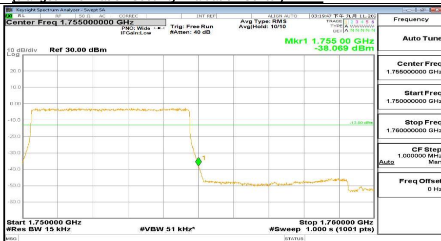
1750MHz-1760MHz_FreqHigh_BW(_5MHz)_RB(25@24)_QPSK_Band4
