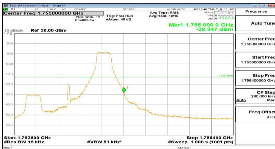
1753.6MHz-1756.4MHz_FreqHigh_BW(_1D4MHz)_RB(1@5)_QPSK_Band4
