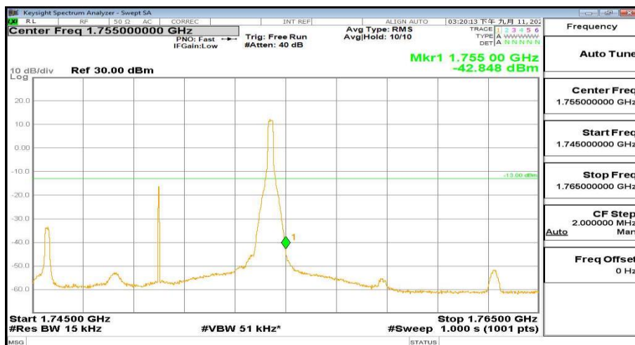
1745MHz-1765MHz_FreqHigh_BW(_10MHz)_RB(1@49)_QPSK_Band4
