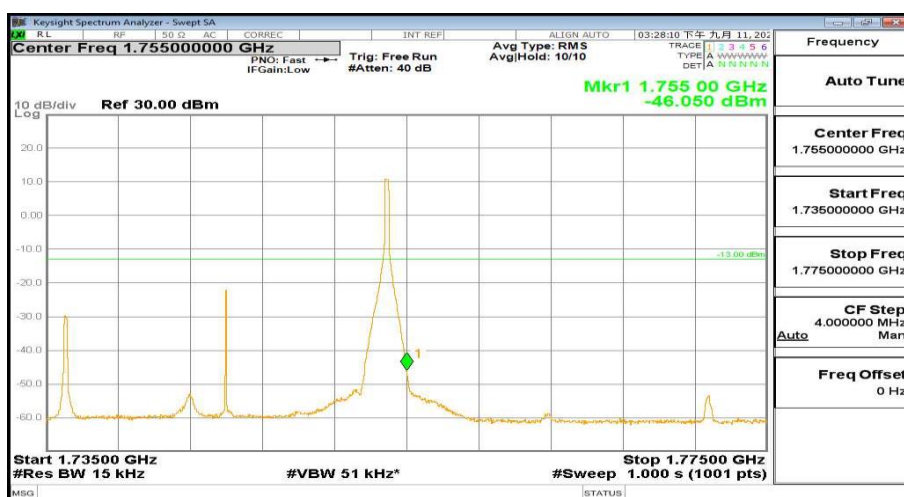
1735MHz-1775MHz_FreqHigh_BW(20MHz)_RB(1@99)_QPSK_Band4
