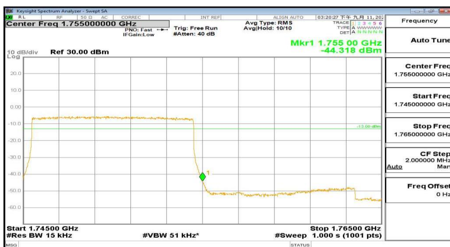
1745MHz-1765MHz_FreqHigh_BW(_10MHz)_RB(50@49)_QPSK_Band4
