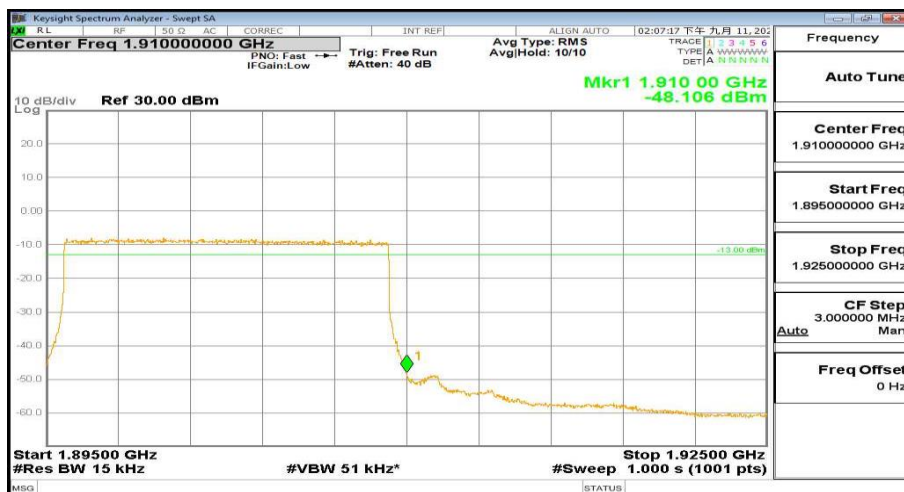
1895MHz-1925MHz_FreqHigh_BW(15MHz)_RB(75@74)_QPSK_Band2
