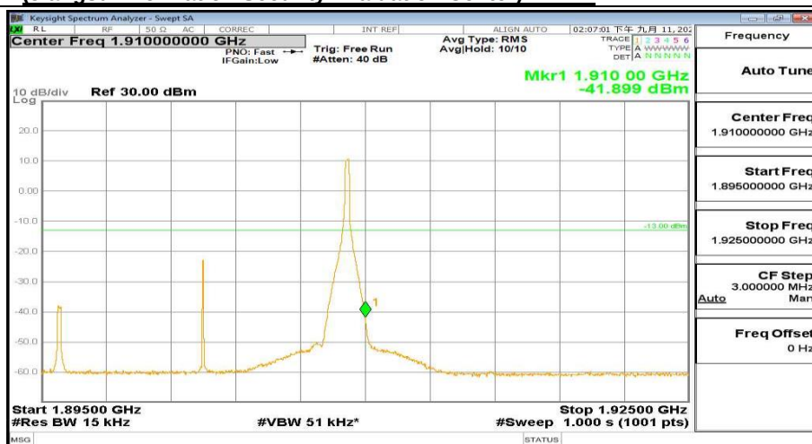
1895MHz-1925MHz_FreqHigh_BW(15MHz)_RB(1@74)_QPSK_Band2
