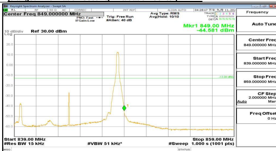
839MHz-859MHz_FreqHigh_BW( 10MHz)_RB(1@49)_QPSK_Band5
