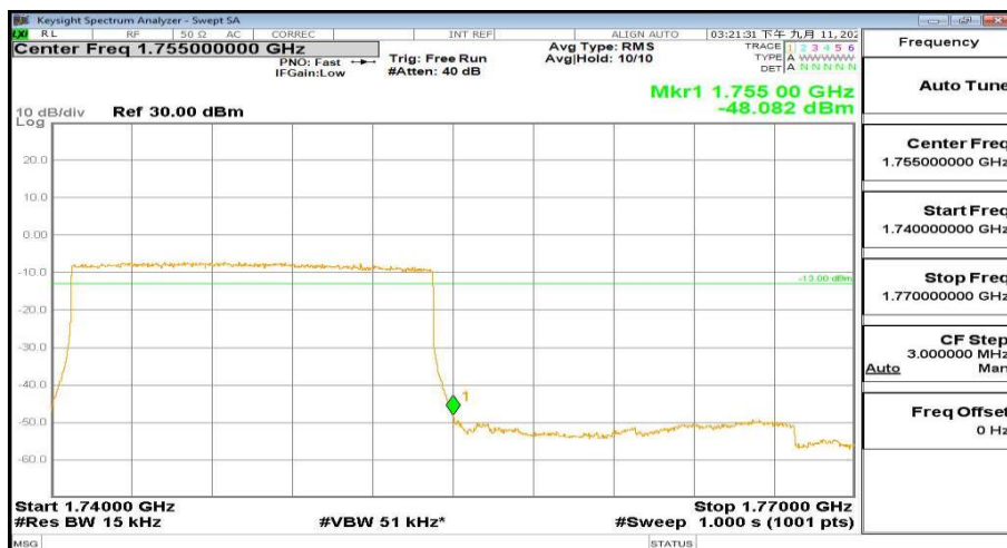
1740MHz-1770MHz_FreqHigh_BW(15MHz)_RB(75@74)_QPSK_Band4
