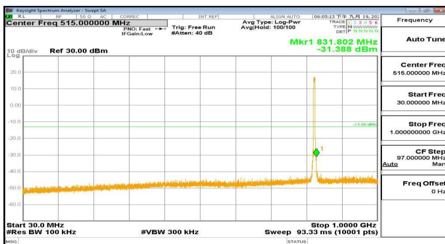
WCDMA Band5 Channel-4132 0.03GHz-1GHz
