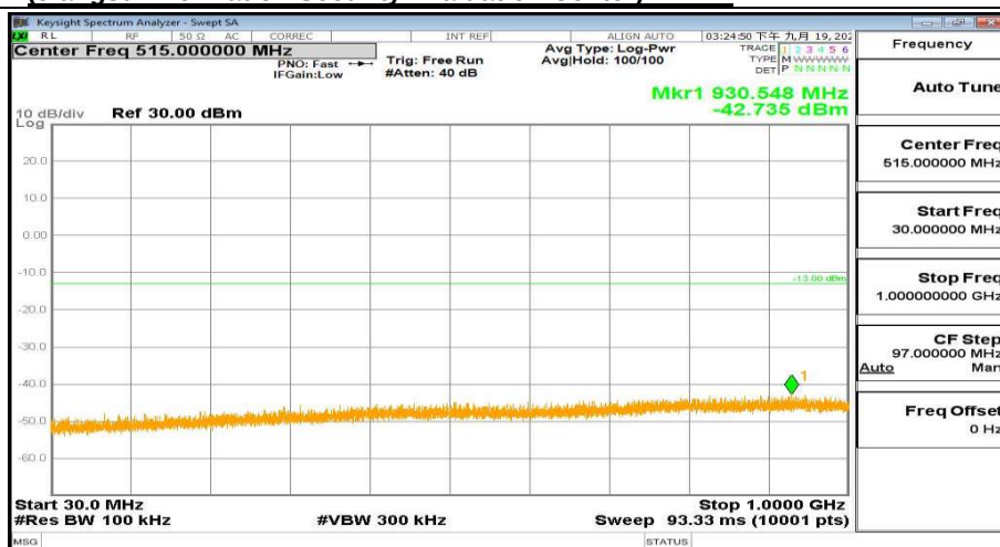
WCDMA Band4 Channel-1413 0.03GHz-1GHz
