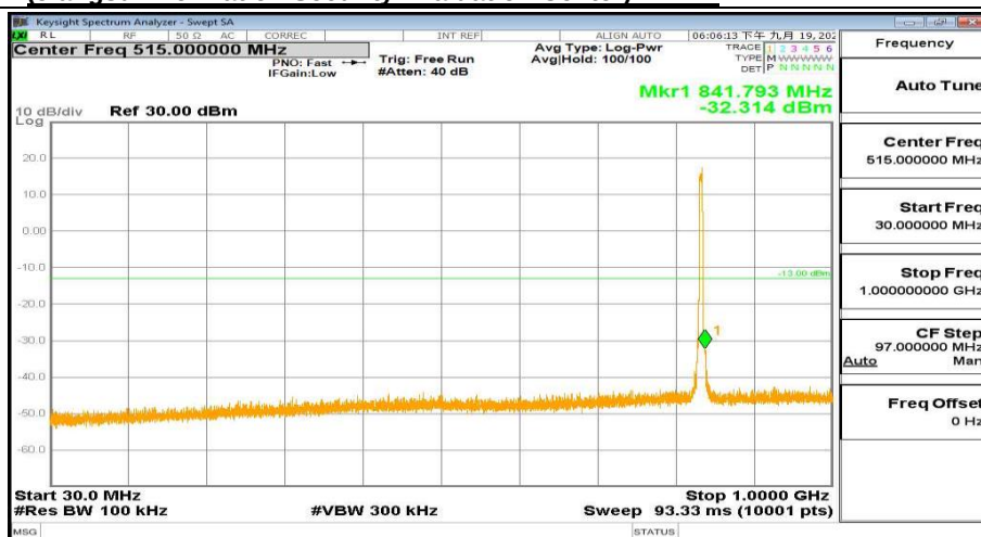
WCDMA Band5 Channel-4182 0.03GHz-1GHz
