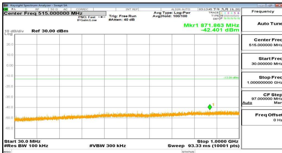
WCDMA Band2 Channel-9262 0.03GHz-1GHz
