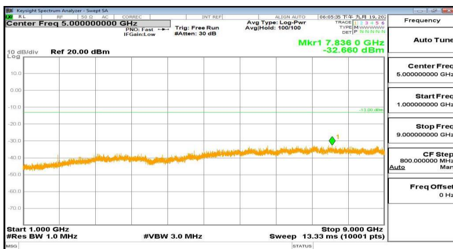
WCDMA Band5 Channel-4132 1GHz-9GHz
