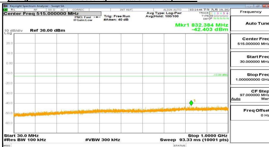
WCDMA Band2 Channel-9400 0.03GHz-1GHz
