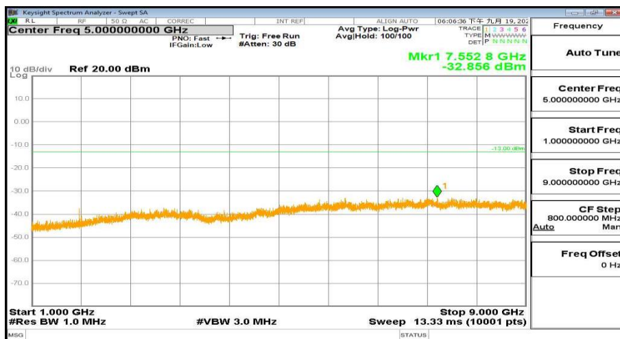
WCDMA Band5 Channel-4182 1GHz-9GHz
