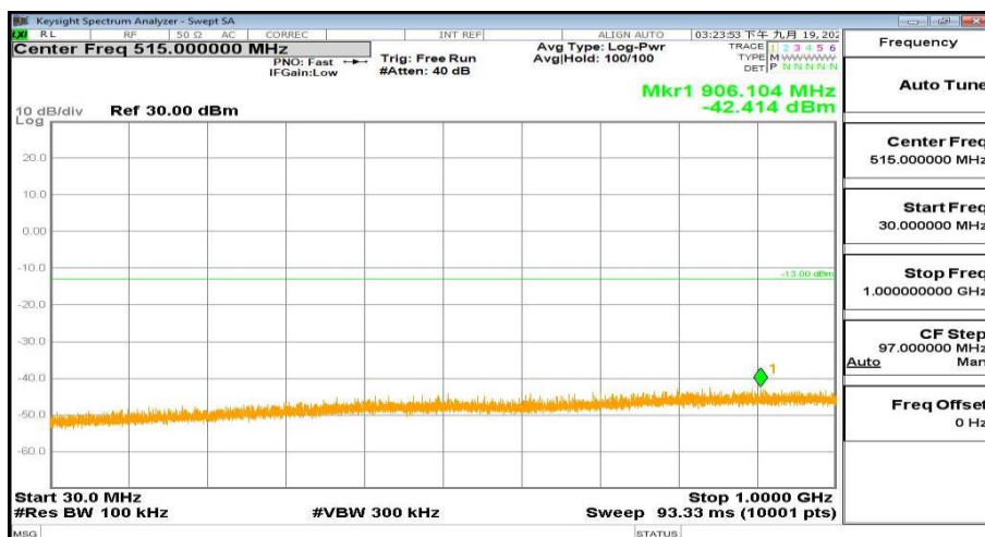
WCDMA Band4 Channel-1312 0.03GHz-1GHz
