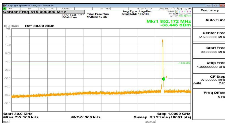
WCDMA Band5 Channel-4233 0.03GHz-1GHz
