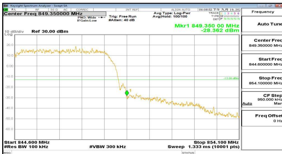
WCDMA Band5 Channel-4233 0.8446GHz-0.8541GHz
