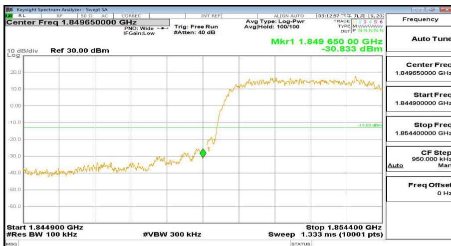
WCDMA Band2 Channel-9262 1.8449GHz-1.8544GHz
