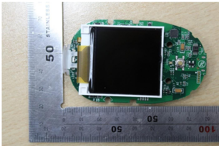
Top side view of PCBA
