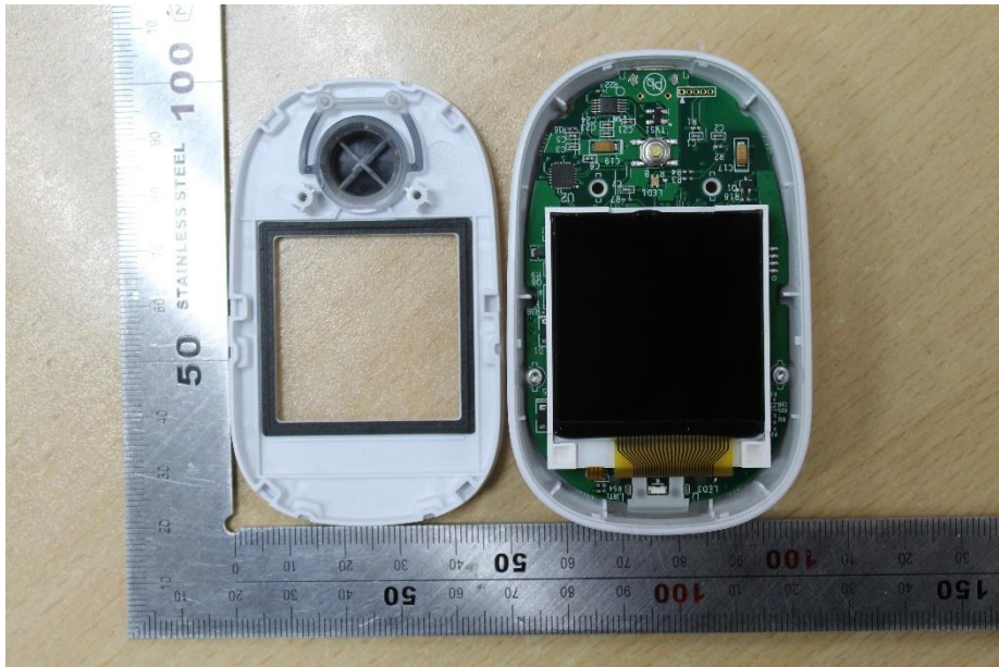
Inner side view of VGM04
