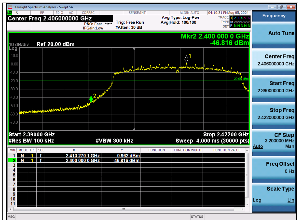
Test Graph 802.11n20 ANT1 2412 MCS0 Lower Band Edge Emissions
