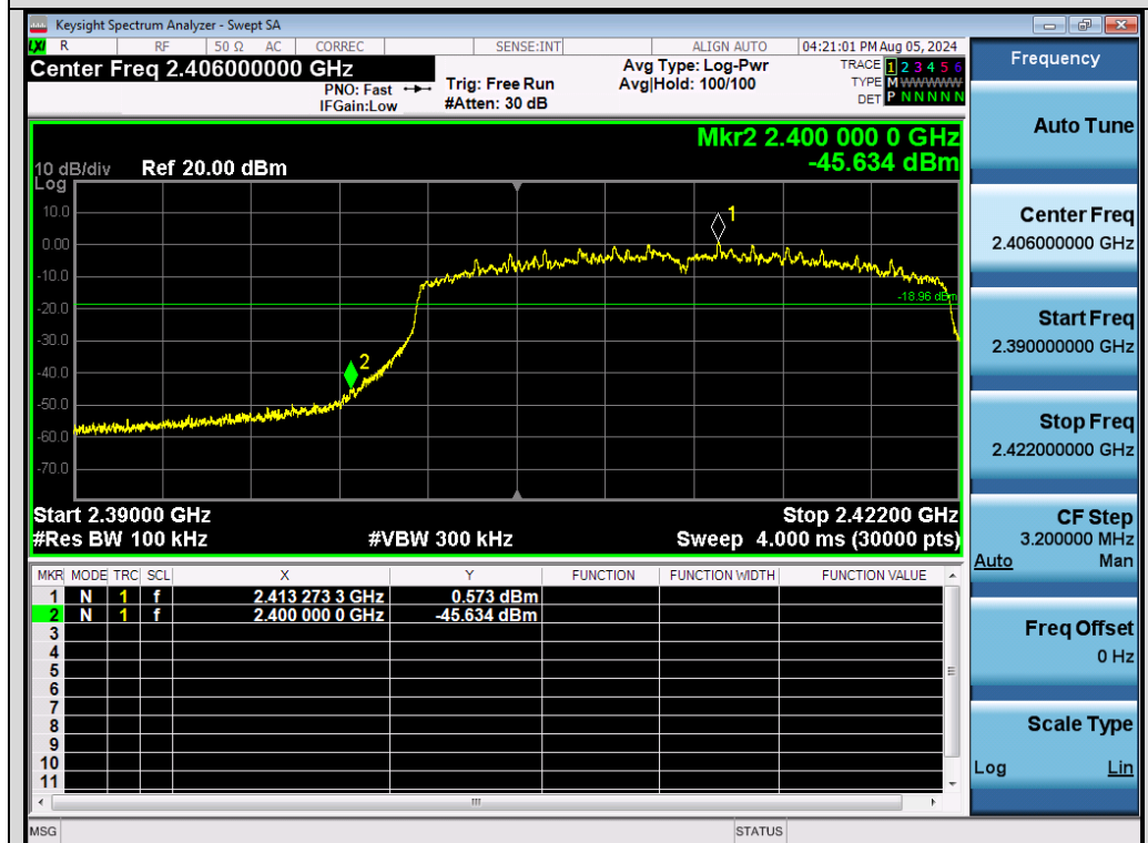
Test Graph 802.11ax20 ANT1 2412 MCS0 Lower Band Edge Emissions
