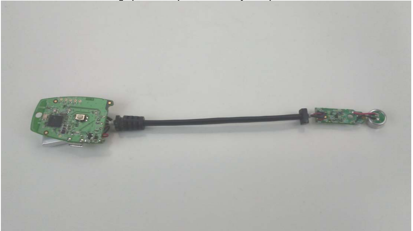
Photograph of Microphone Assembly: Battery Side
