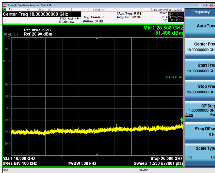
RF Conducted Spurious Emissions_3DH5_2441
