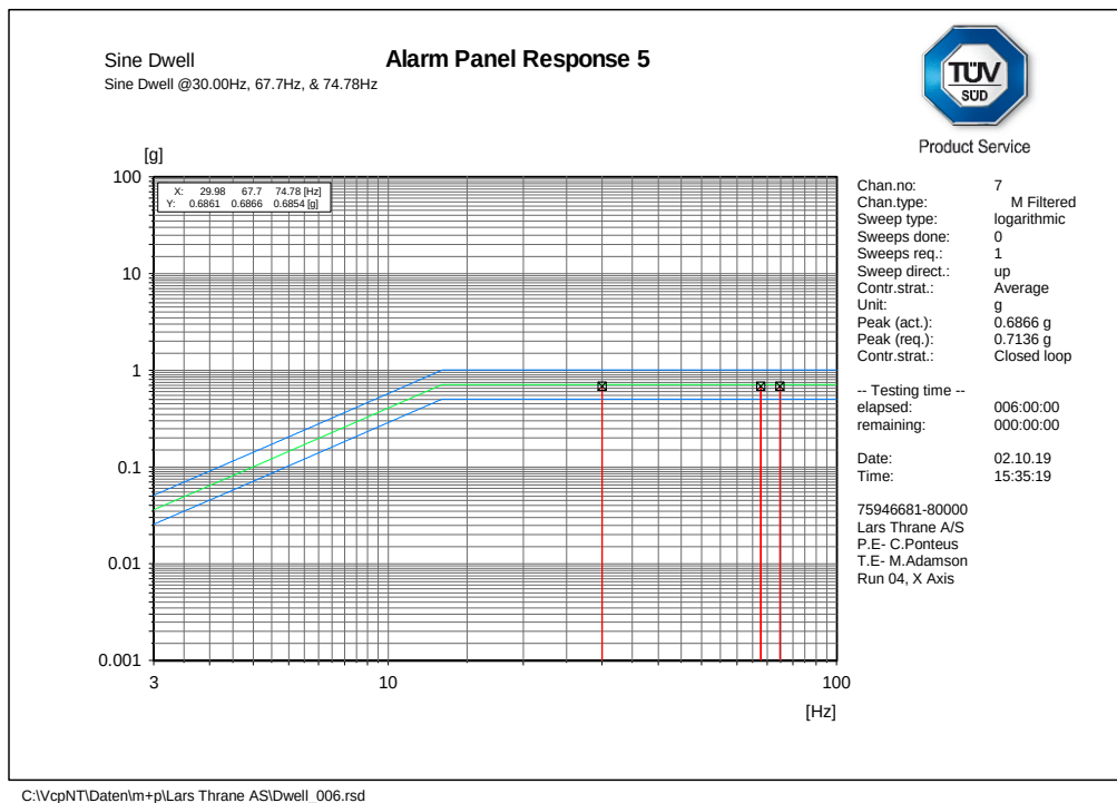
Figure 2.8.9 Run 04, X axis, Dwell
