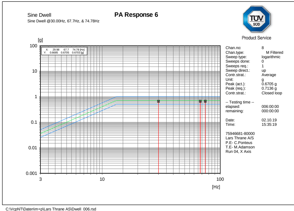
Figure 2.8.10 Run 04, X axis, Dwell
