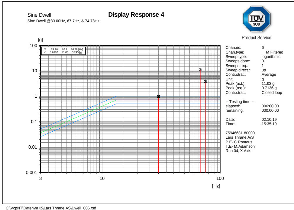
Figure 2.8.8 Run 04, X axis, Dwell
