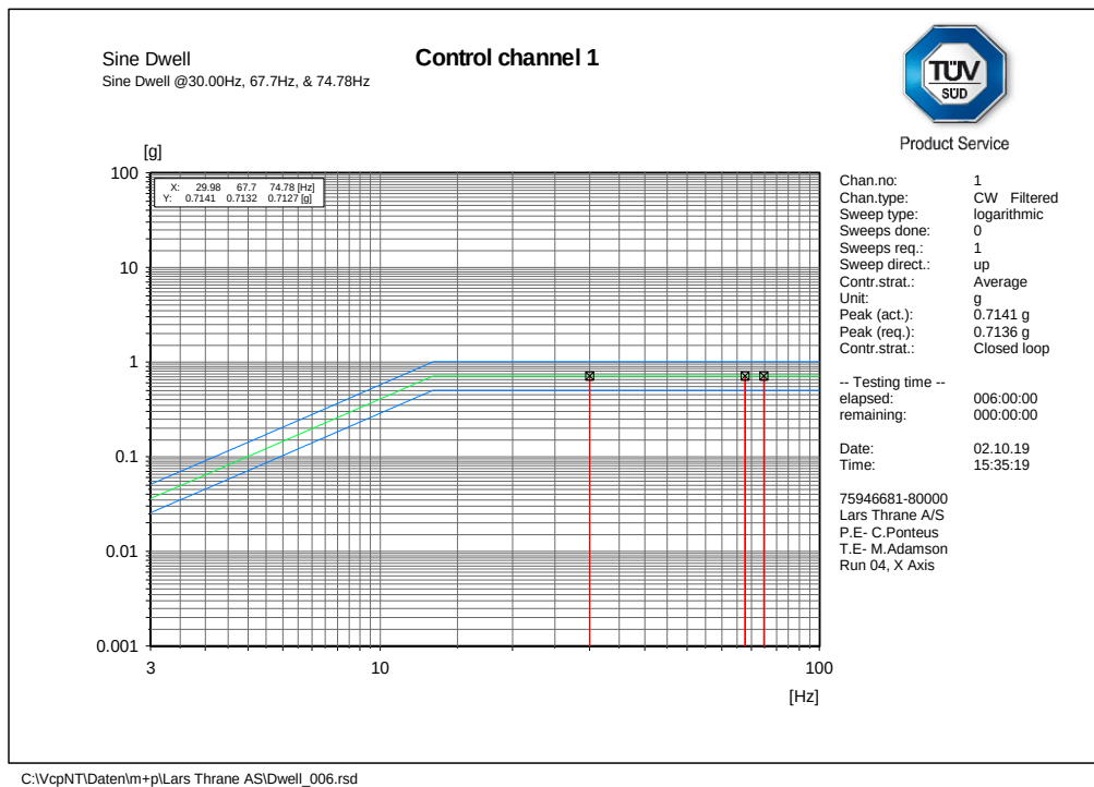
Figure 2.8.11 Run 04, X axis, Dwell
