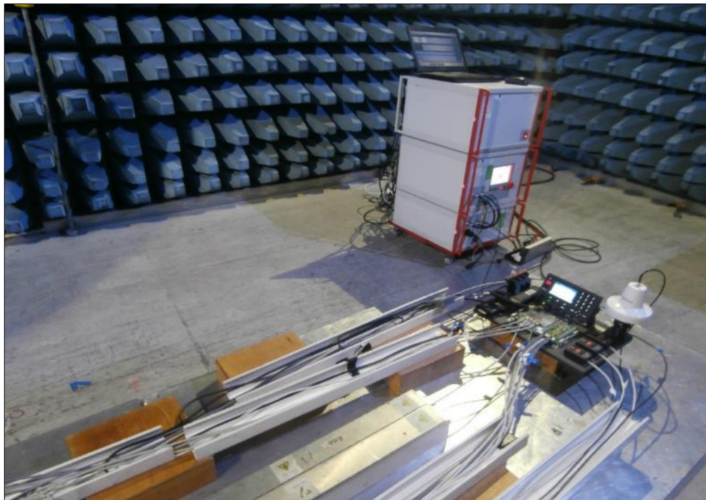
Figure 22 - Test Setup
