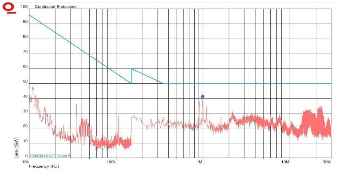
Figure 13 - Graphical Results
