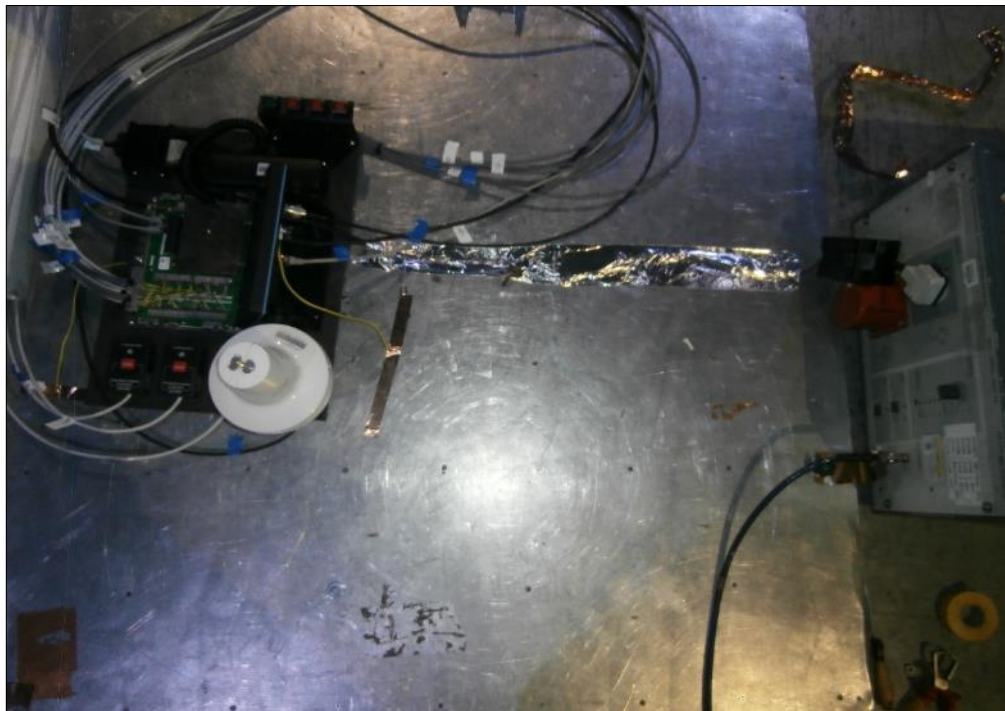
Figure 14 - Test Setup
