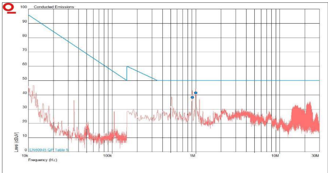
Figure 12 - Graphical Results
