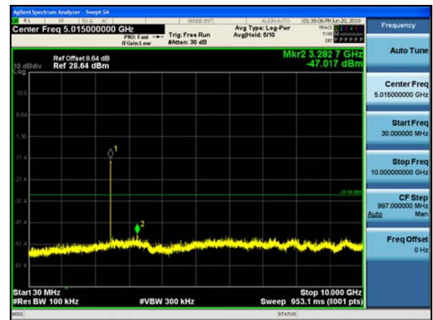
Spurious emission
