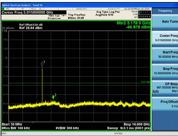
Spurious emission
