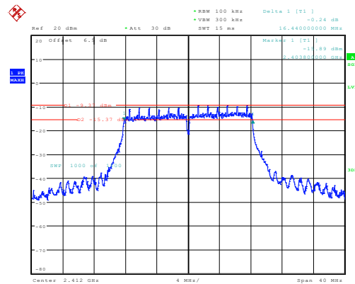
g_2412MHz_Chain 0 16.440MHz
