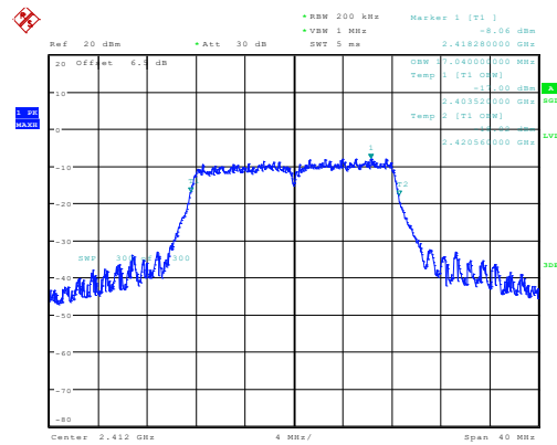
g_2412MHz_Chain 0 17.040MHz
