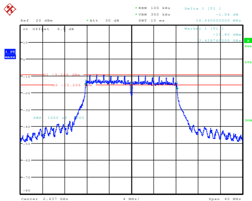
g_2437MHz_Chain 0 16.440MHz
