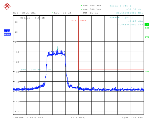
n20_2462MHz_Chain 0 37.37dB
