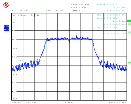
g_2462MHz_Chain 0 16.840MHz
