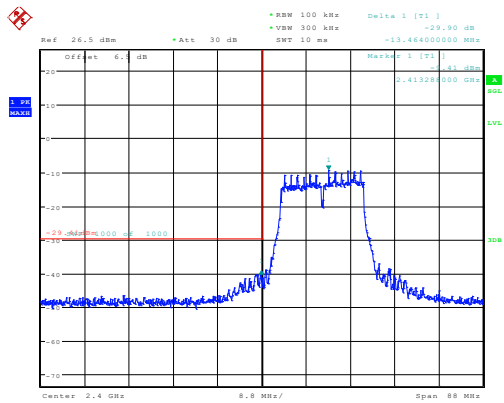
g_2412MHz_Chain 0 29.90dB
