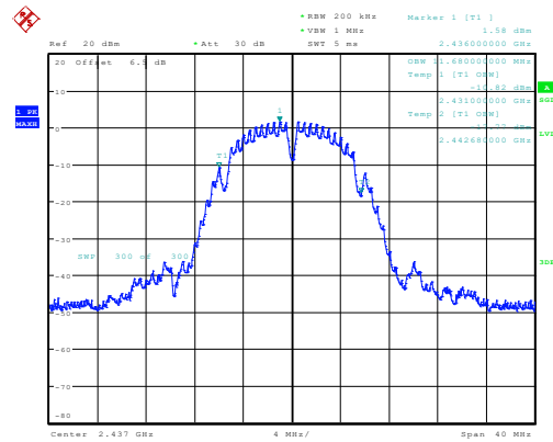
b_2437MHz_Chain 0 11.680MHz
