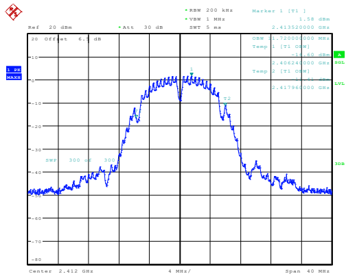
b_2412MHz_Chain 0 11.720MHz
