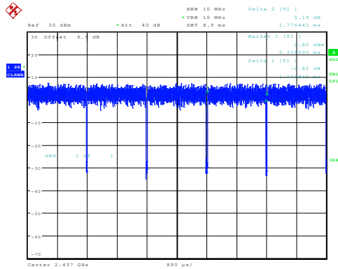
n20_2437MHz_Chain 0 1.741ms,1.776ms
