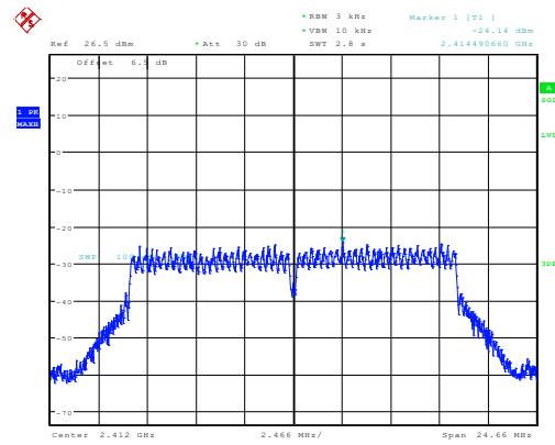
g_2412MHz_Chain 0 -24.14dBm/3kHz
