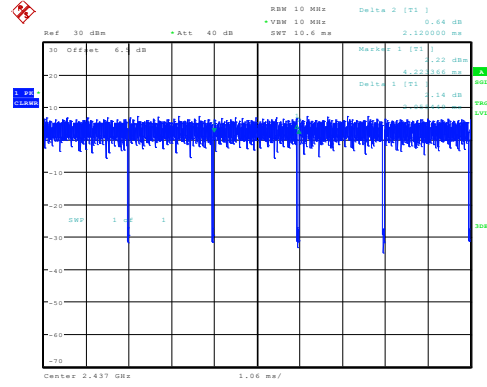
g_2437MHz_Chain 0 2.055ms,2.120ms
