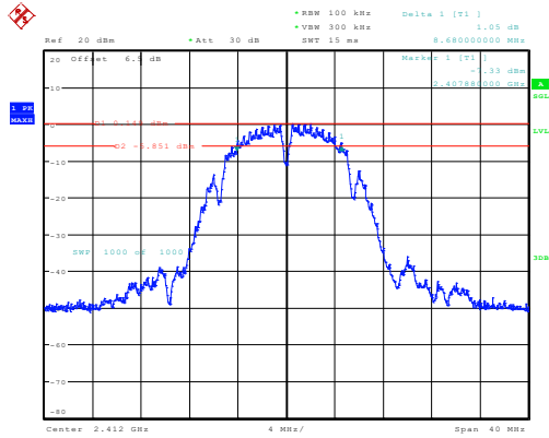
b_2412MHz_Chain 0 8.680MHz
