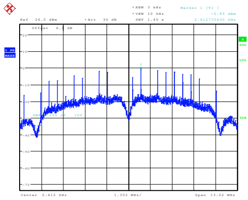
b_2412MHz_Chain 0 -0.85dBm/3kHz
