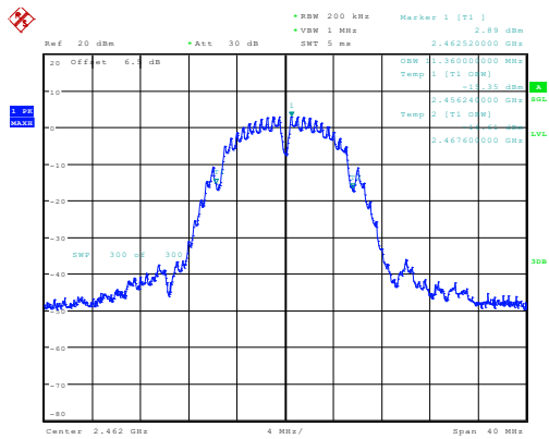
b_2462MHz_Chain 0 11.360MHz
