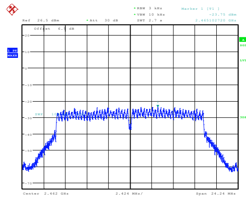
g_2462MHz_Chain 0 -23.75dBm/3kHz
