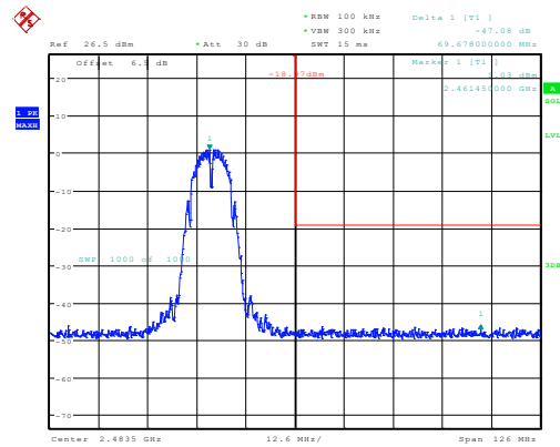
b_2462MHz_Chain 0 47.08dB
