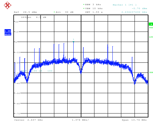
b_2437MHz_Chain 0 -0.70dBm/3kHz
