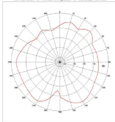
Far-field Power Distribution(H+V) on X-Z Plane Plot Peak Gain(H+V)= 1.04 dB; Plot AvgGain(H+V)= -3.83dB @2.44000 GHz
